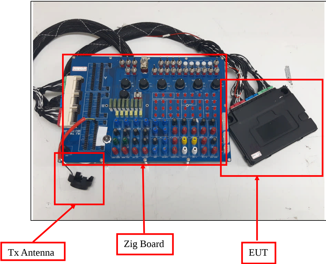
View of Test Zig and EUT
