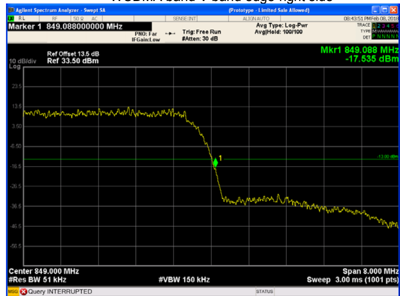
WCDMA band V band edge-right side
