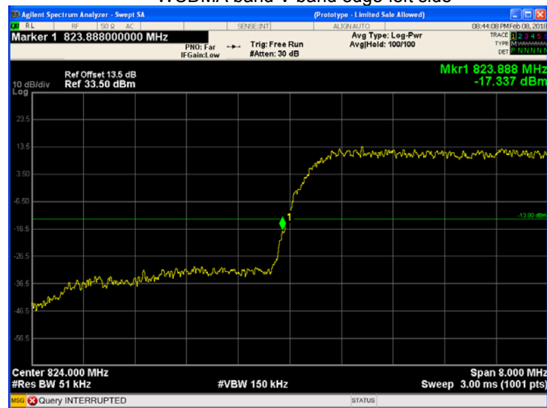
WCDMA band V band edge-left side
