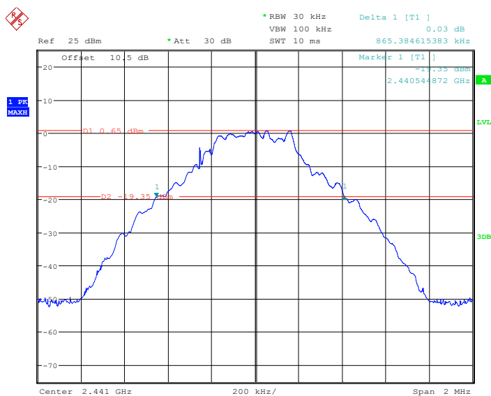
DH5_2441MHz
