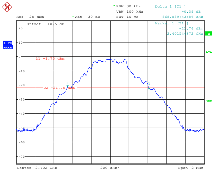
DH5_2402MHz
