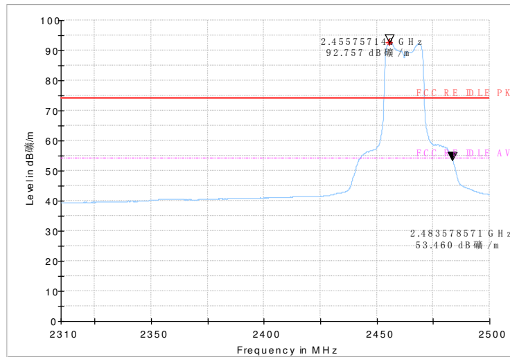
Fig.65 Radiated emission (Power): 802.11g, channel 11
