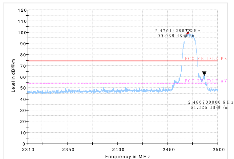
Fig.61 Radiated emission (Power): 802.11b, channel 12
