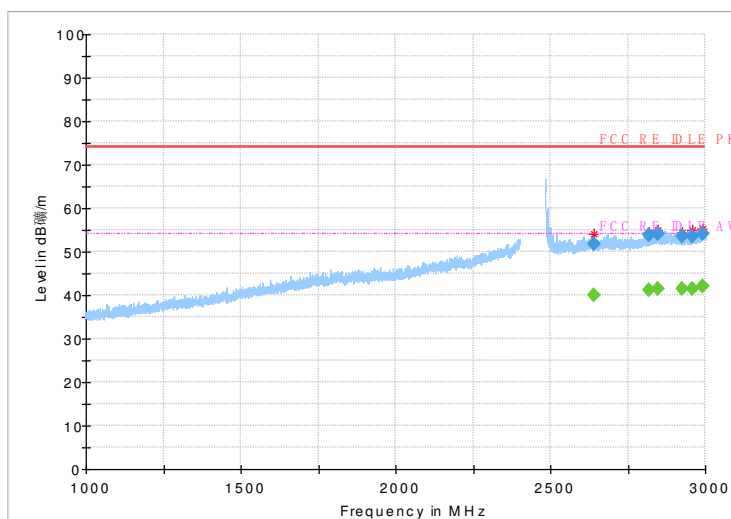
Fig.84 Radiated Spurious Emission (802.11g,Ch11,1GHz~3GHz)
