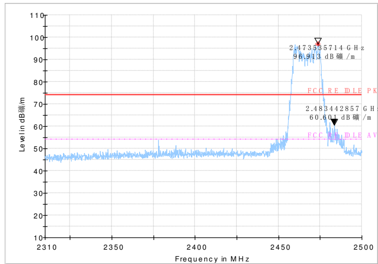
Fig.69 Radiated emission (Power): 802.11g, channel 12
