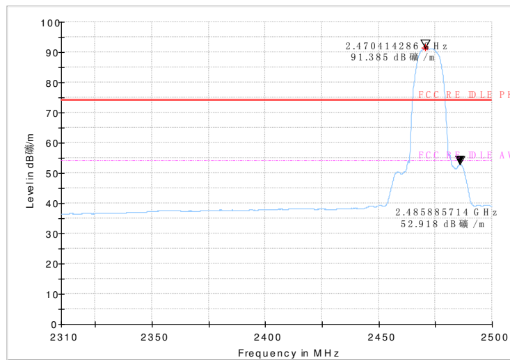
Fig.87 Radiated emission (Power): 802.11g, channel13
