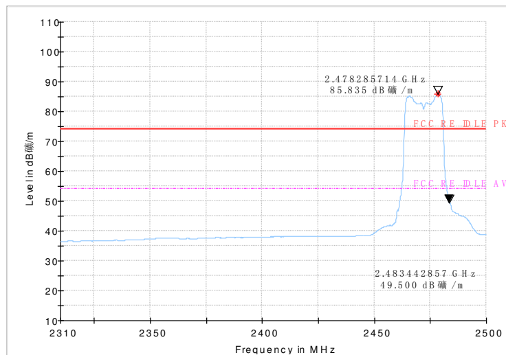
Fig.72 Radiated emission (Power): 802.11g, channel 13
