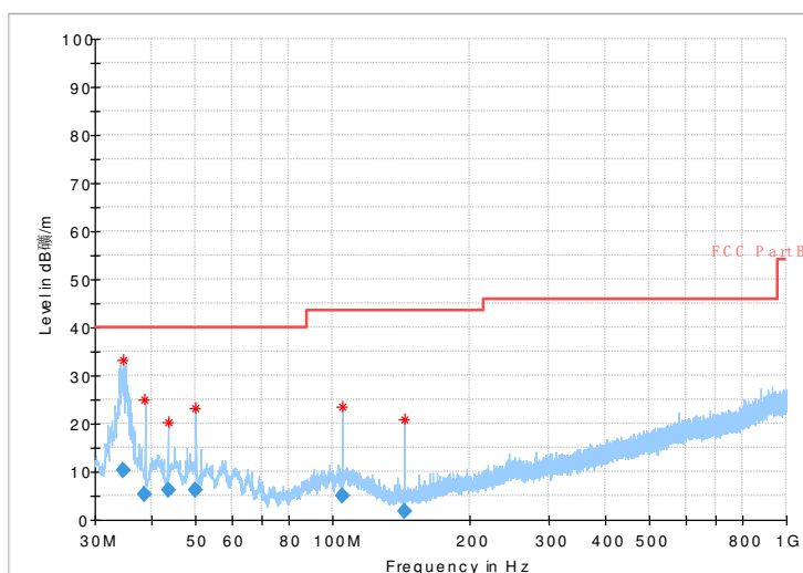
Fig.83 Radiated Spurious Emission (802.11 g,Ch11,30MHz~1GHz)
