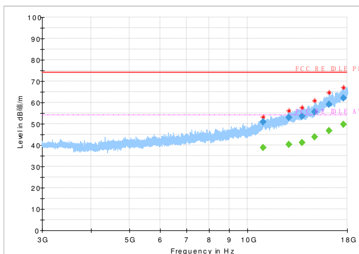
Fig.85 Radiated Spurious Emission (802.11g,Ch11,3GHz~18GHz)
