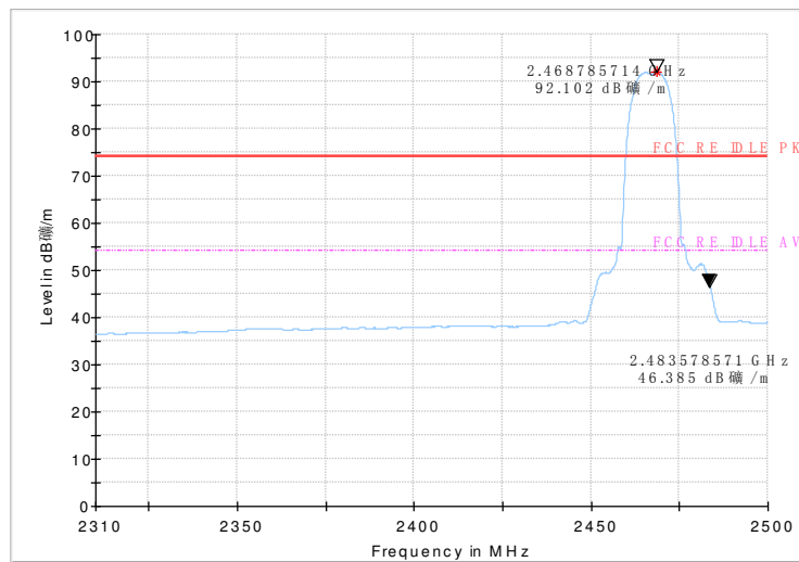
Fig.86 Radiated emission (Power): 802.11g, channel12
