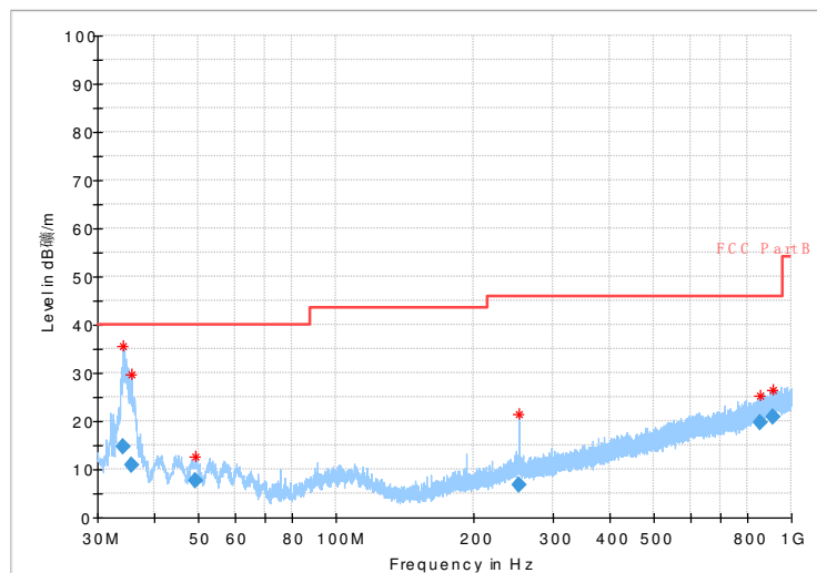
Fig.66 Radiated Spurious Emission (802.11g,Ch11,30MHz~1GHz)
