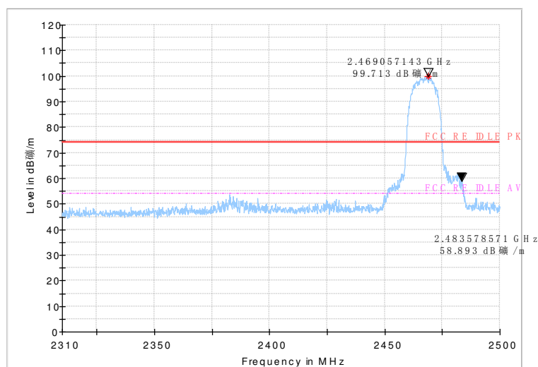
Fig.60 Radiated emission (Power): 802.11b, channel 12
