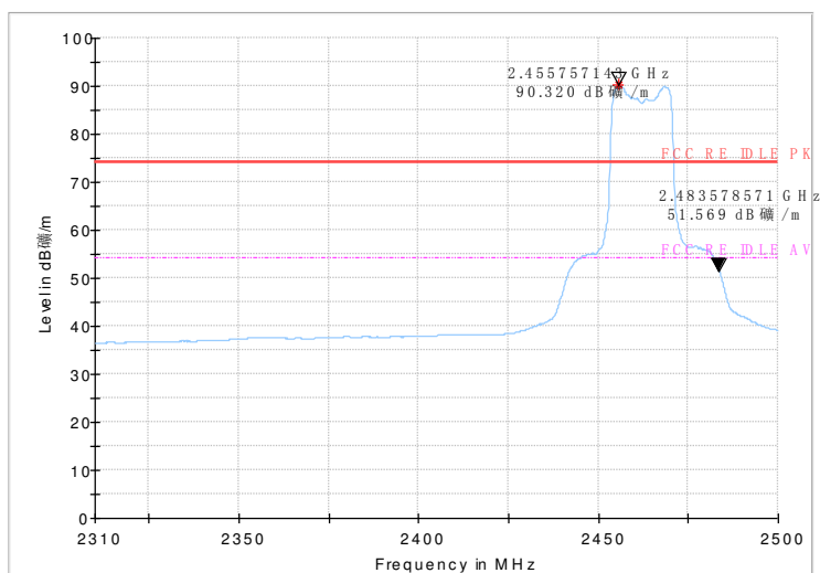
Fig.82 Radiated emission (Power): 802.11g, high channel
