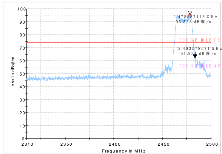
Fig.71 Radiated emission (Power): 802.11g, channel 13
