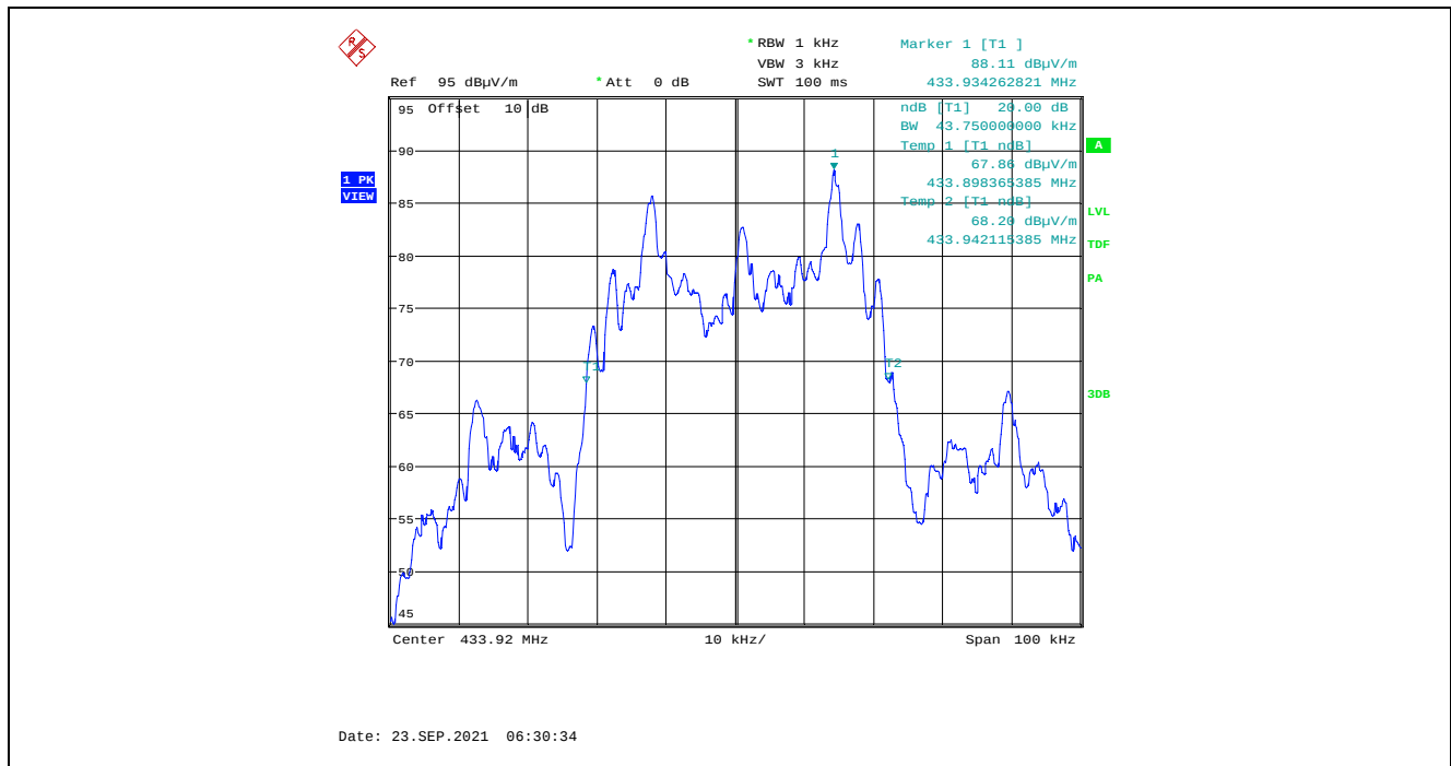
Plot 5.3.3.3. 20 dB Bandwidth, Fc: 433.92 MHz FSK modulated with programmed messages (SM6)
