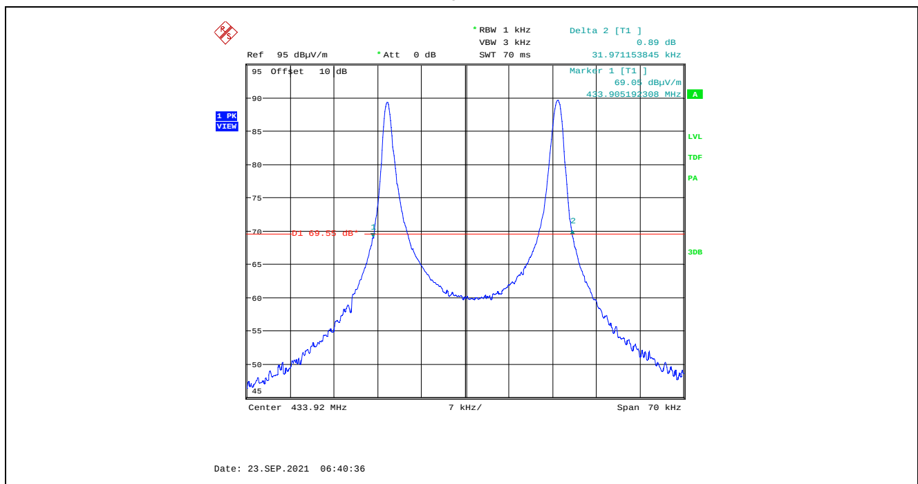
Plot 5.3.3.4. 20 dB Bandwidth, Fc: 433.92 MHz FSK modulated with a signal 101010..., 1 b/s (SM5)
