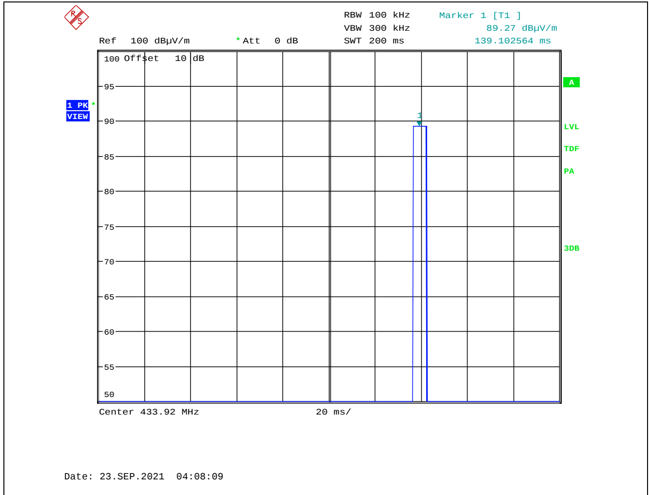
Plot 5.2.3.3.2. Duty Cycle (200 ms)
