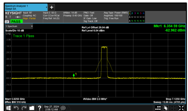
Figure 353 - B (Core 1) 802.11ax HE40 SU VLP 6565 MHz (CH123)
