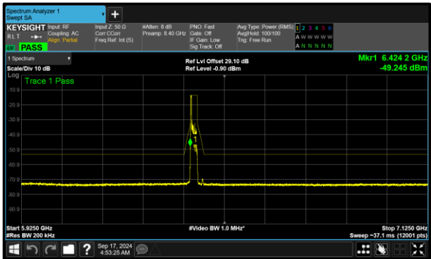
Figure 343 - B (Core 1) 802.11ax HE20 RU26 LPI 6435 MHz (CH97)
