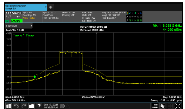
Figure 348 - B (Core 1) 802.11ax HE160 SU SP 6345 MHz (CH79)
