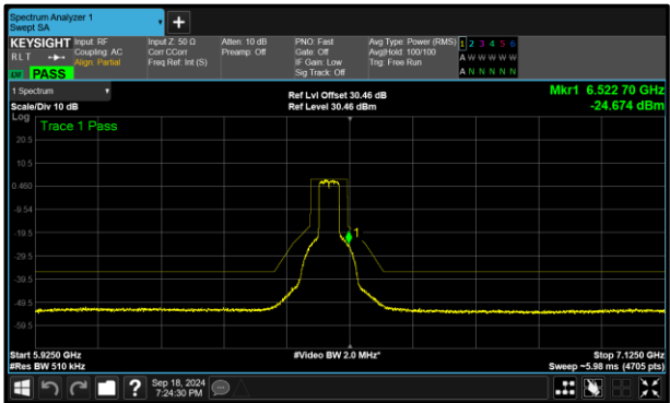
Figure 361 - A (Core 0) 802.11ax HE40 SU SP 6485 MHz (CH107)
