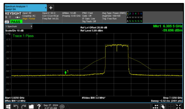
Figure 355 - B (Core 1) 802.11ax HE160 SU VLP 6665 MHz (CH143)
