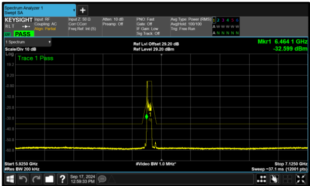
Figure 350 - B (Core 1) 802.11ax HE20 RU26 SP 6475 MHz (CH105)
