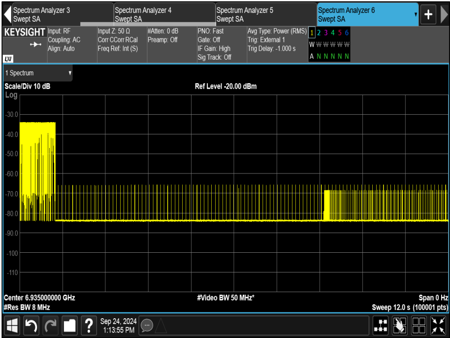
Figure 379 - U-NII-8, Maximum Bandwidth (AWGN Low)
