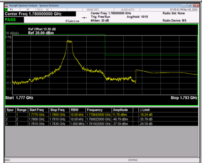
Band66-1.4MHz-64QAM-132665-6RB#0
