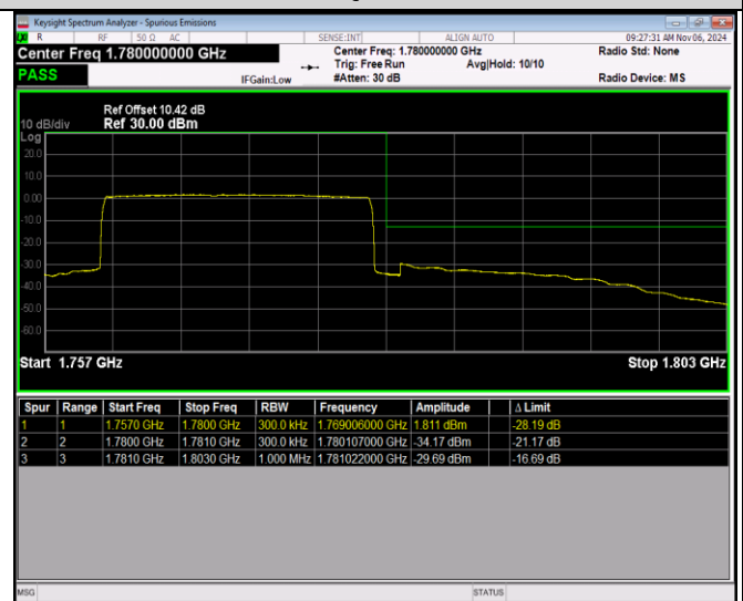
Band66-20MHz-64QAM-132572-100RB#0
