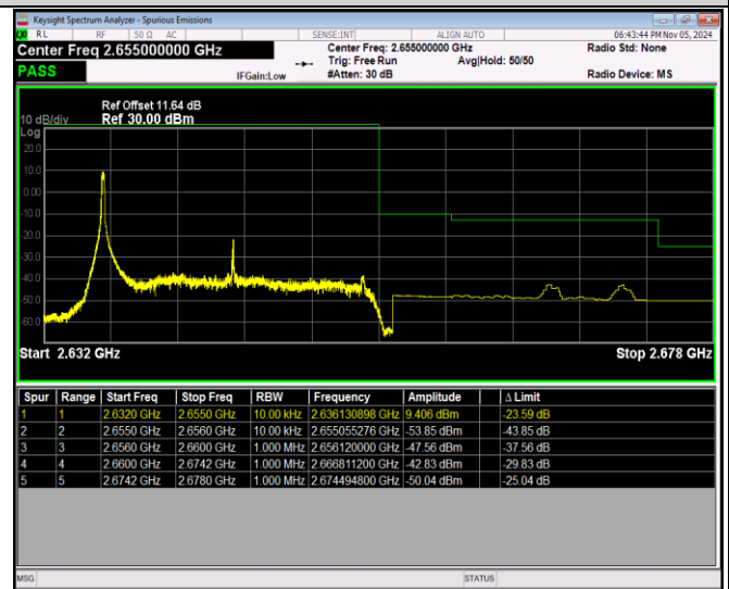
Band41-20MHz-16QAM-41140-100RB#0
