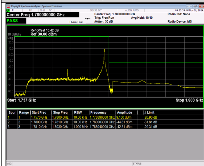
Band66-20MHz-64QAM-132572-1RB#99
