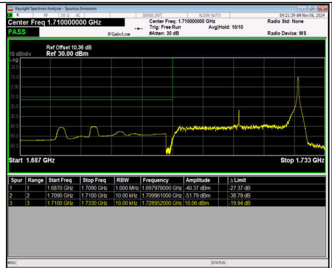
Band66-20MHz-16QAM-132572-1RB#0
