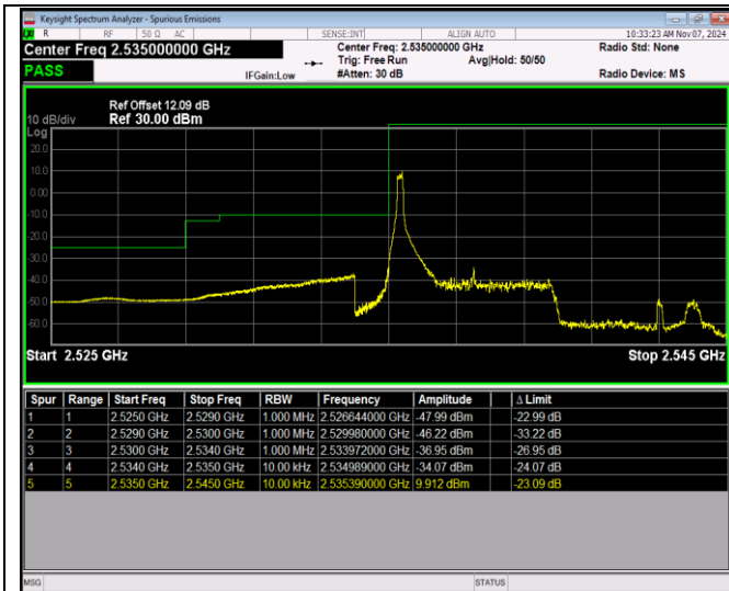
Band41-5MHz-16QAM-40065-25RB#0
