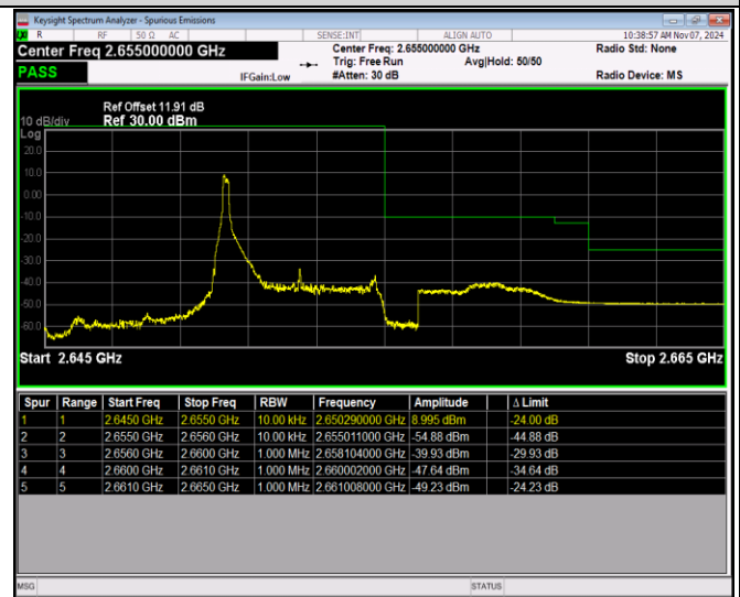
Band41-5MHz-64QAM-41215-25RB#0
