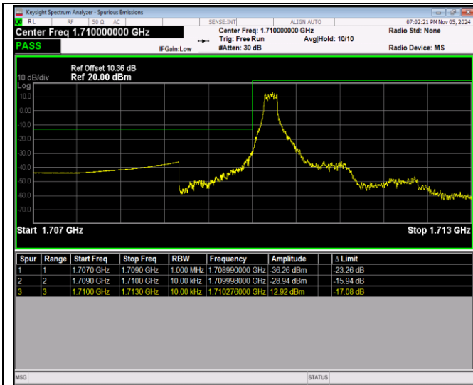
Band66-1.4MHz-16QAM-131979-6RB#0
