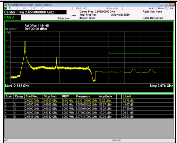
Band41-20MHz-QPSK-41140-100RB#0
