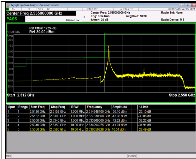
Band41-20MHz-16QAM-40140-100RB#0
