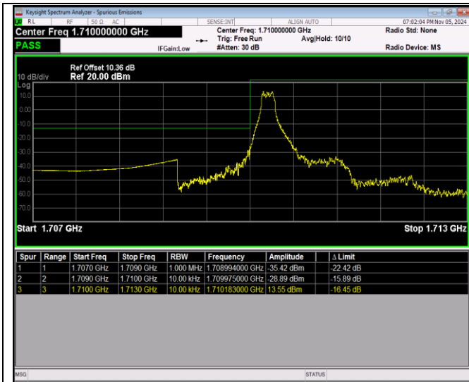
Band66-1.4MHz-QPSK-131979-6RB#0
