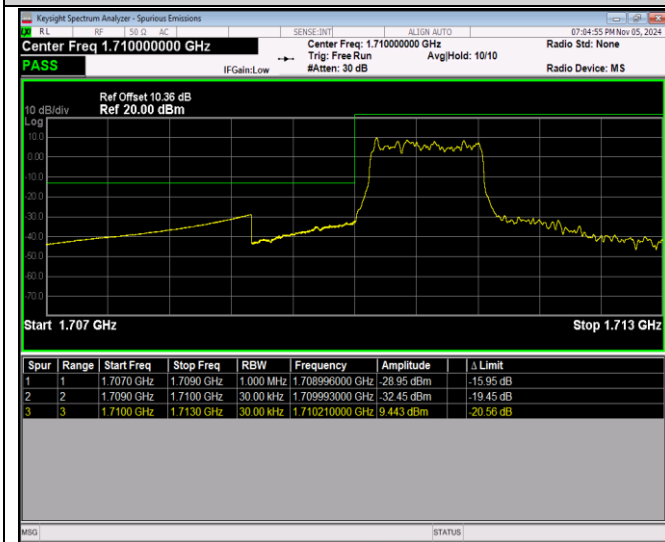
Band66-1.4MHz-64QAM-132665-1RB#5
