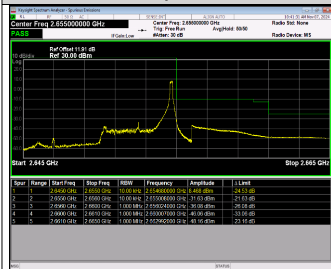
Band41-5MHz-64QAM-40065-1RB#0
