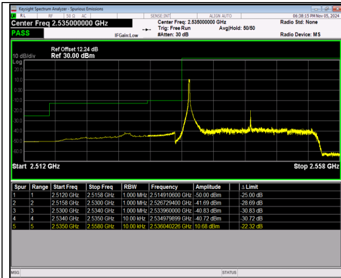
Band41-20MHz-QPSK-40140-100RB#0
