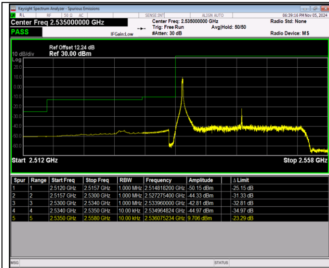
Band41-20MHz-64QAM-40140-100RB#0
