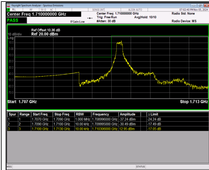
Band66-1.4MHz-64QAM-131979-6RB#0
