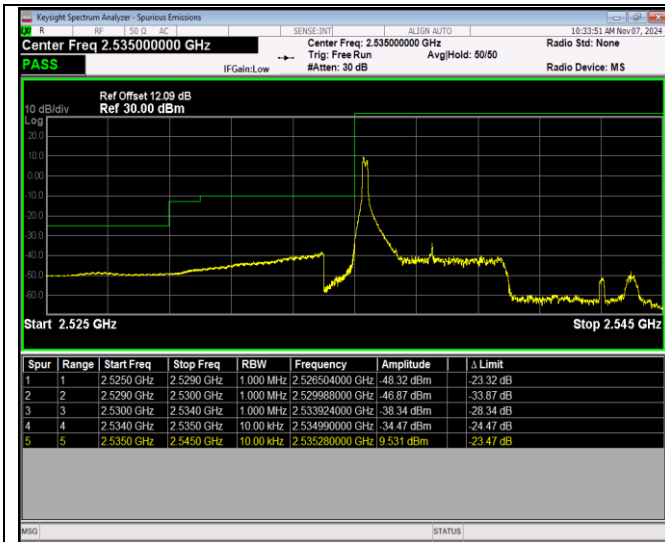
Band41-5MHz-64QAM-40065-25RB#0
