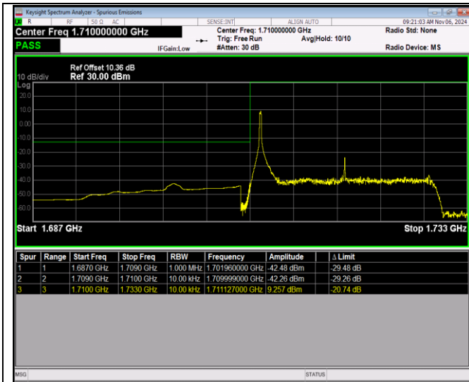
Band66-20MHz-64QAM-132072-100RB#0
