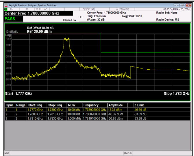
Band66-1.4MHz-16QAM-132665-6RB#0
