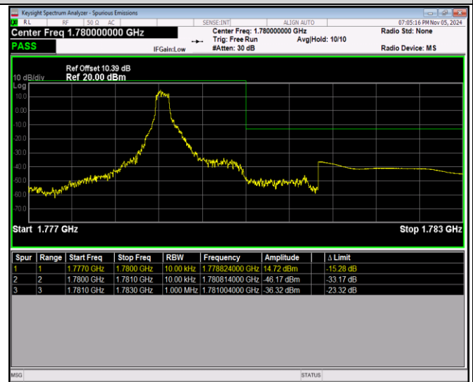
Band66-1.4MHz-QPSK-132665-6RB#0
