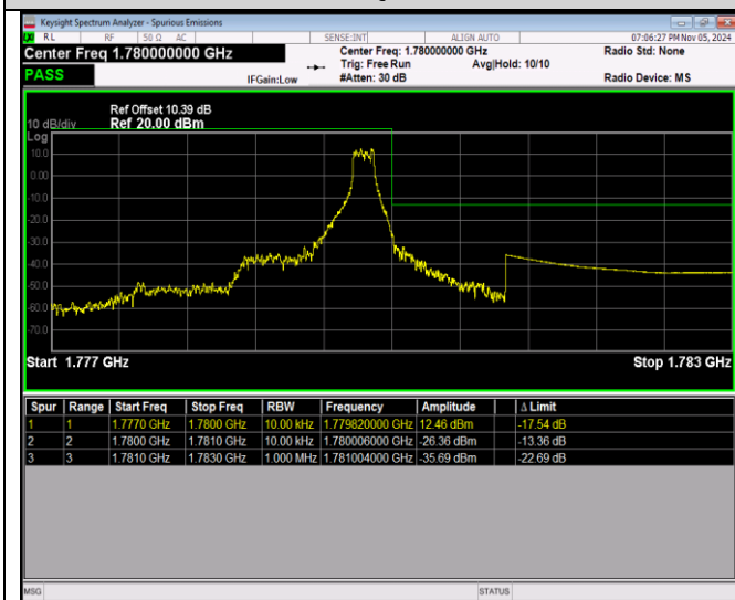
Band66-1.4MHz-64QAM-131979-1RB#0
