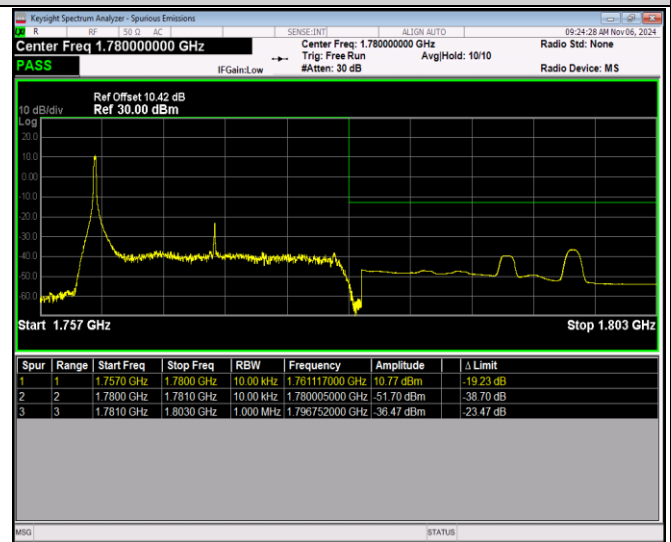
Band66-20MHz-16QAM-132572-100RB#0
