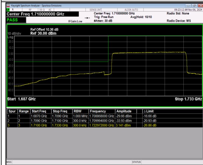
Band66-20MHz-16QAM-132572-1RB#99
