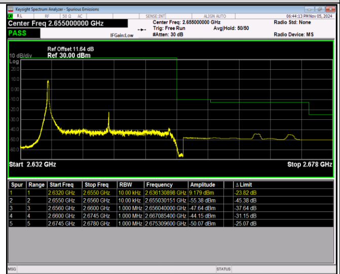
Band41-20MHz-64QAM-41140-100RB#0
