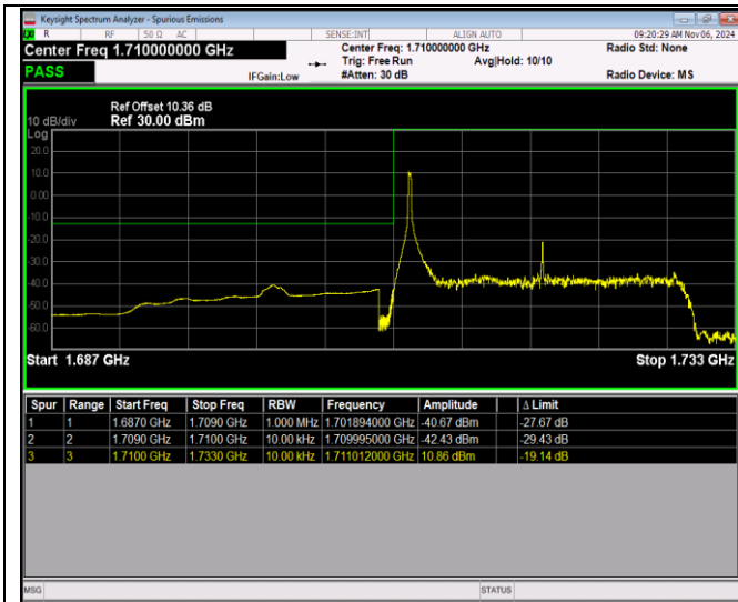
Band66-20MHz-QPSK-132072-100RB#0
