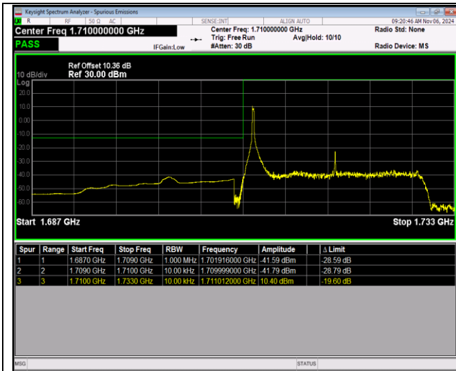
Band66-20MHz-16QAM-132072-100RB#0
