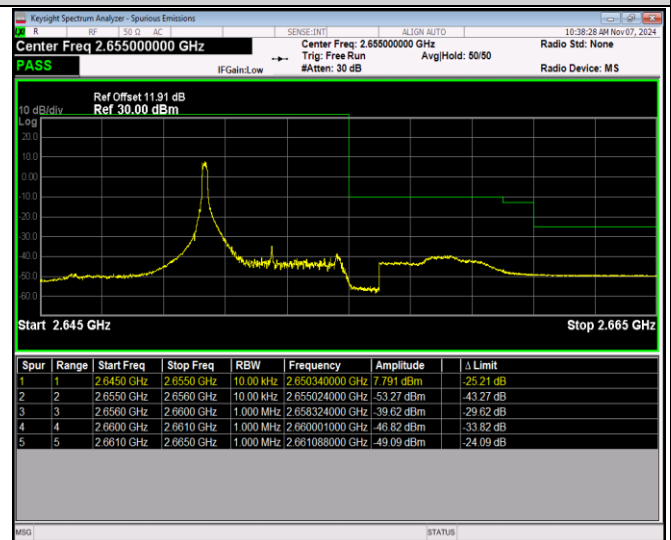
Band41-5MHz-16QAM-41215-25RB#0
