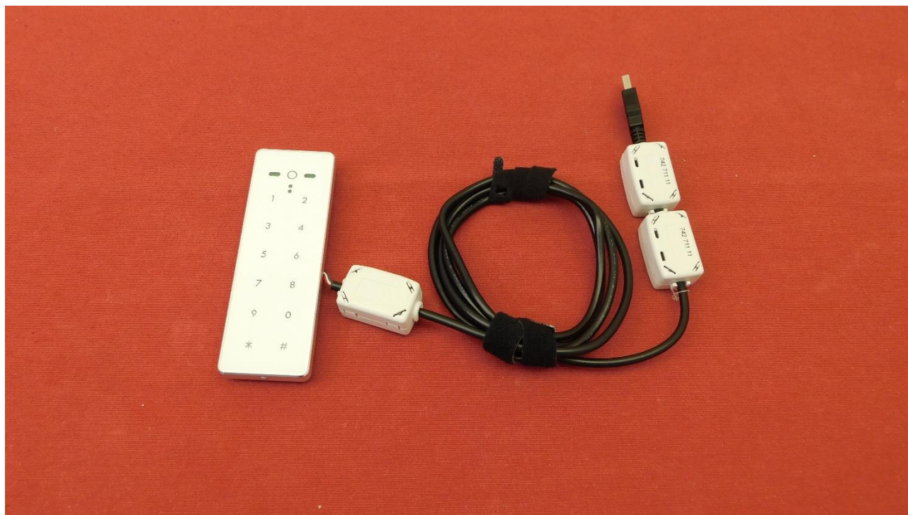
Picture 13: EUT connected with USB cable front view
