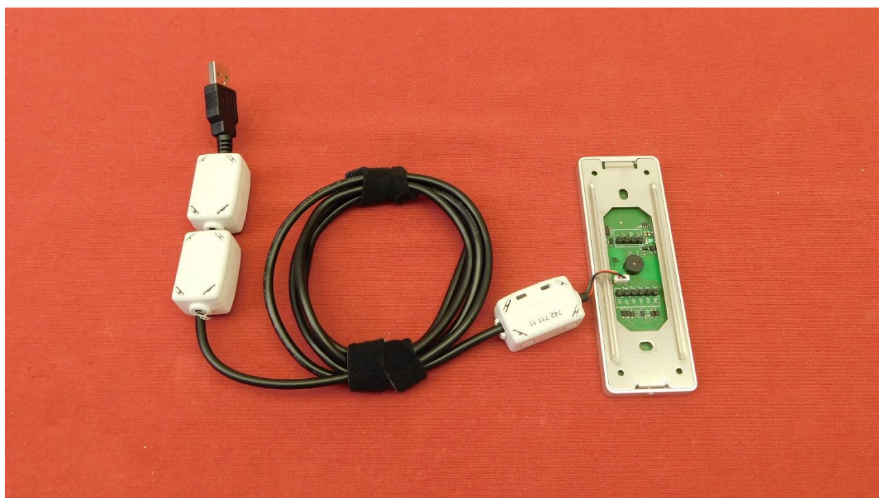
Picture 14: EUT connected with USB cable rear view
