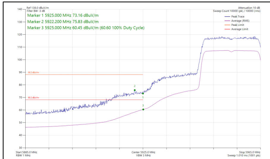
Figure 97 - 802.11ax HE20, SU, SISO, Core 0 - 5955 MHz Band Edge Frequency 5925 MHz
