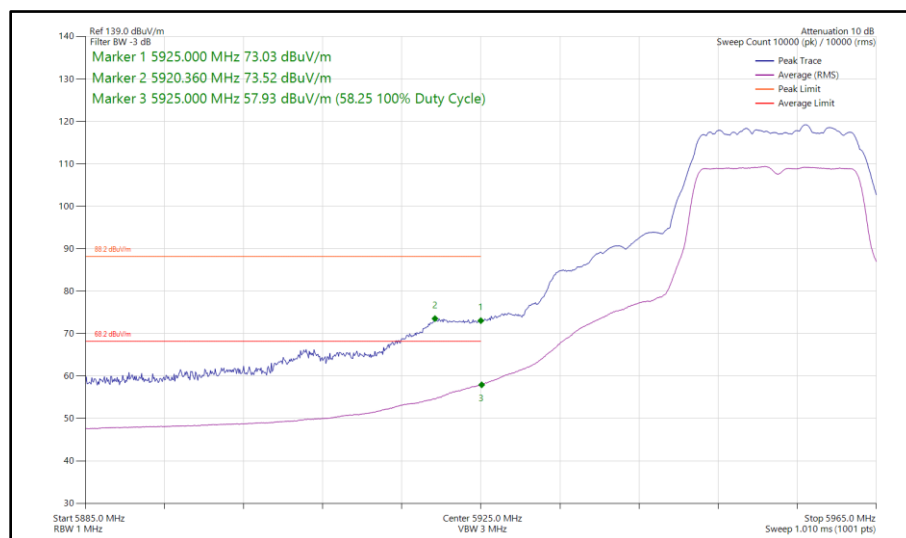
Figure 96 - 802.11a, SISO, Core 0 - 5955 MHz Band Edge Frequency 5925 MHz
