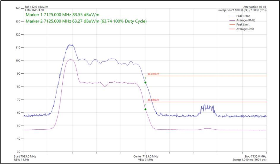
Figure 111 - 802.11ax HE20, RU 26-0, SISO, Core 1 - 7115 MHz Band Edge Frequency 7125 MHz
