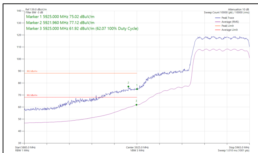
Figure 112 - 802.11ax HE20, SU, CDD, Core 0 - Core 1 - 5955 MHz Band Edge Frequency 5925 MHz
