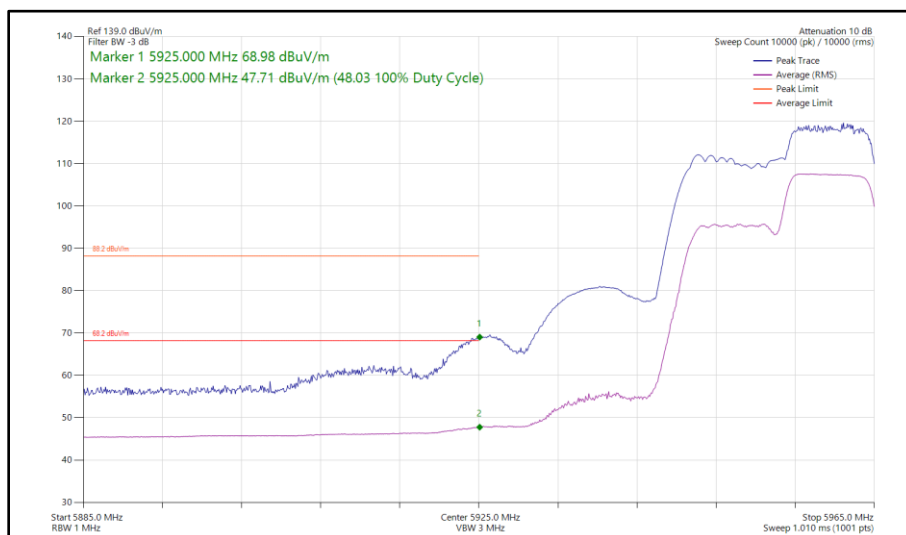
Figure 106 - 802.11ax HE20, RU 106-54, SISO, Core 1 - 5955 MHz Band Edge Frequency 5925 MHz
