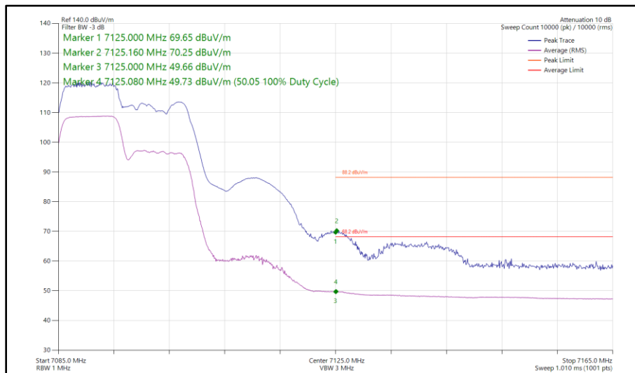
Figure 102 - 802.11ax HE20, RU 106-53, SISO, Core 0 - 7095 MHz Band Edge Frequency 7125 MHz
