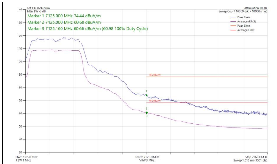
Figure 107 - 802.11a, SISO, Core 1 - 7095 MHz Band Edge Frequency 7125 MHz
