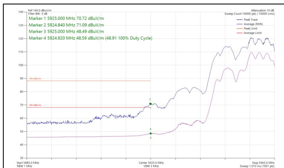
Figure 113 - 802.11ax HE20, RU 106-54, CDD, Core 0 - Core 1 - 5955 MHz Band Edge Frequency 5925 MHz
