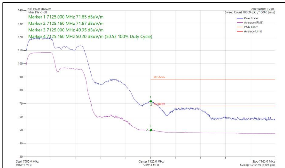
Figure 110 - 802.11ax HE20, RU 106-53, SISO, Core 1 - 7095 MHz Band Edge Frequency 7125 MHz
