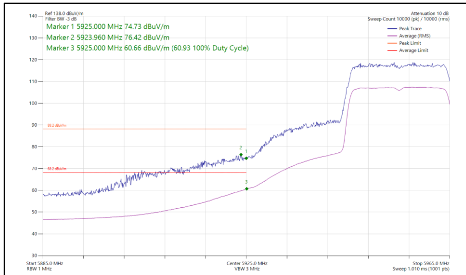
Figure 105 - 802.11ax HE20, SU, SISO, Core 1 - 5955 MHz Band Edge Frequency 5925 MHz
