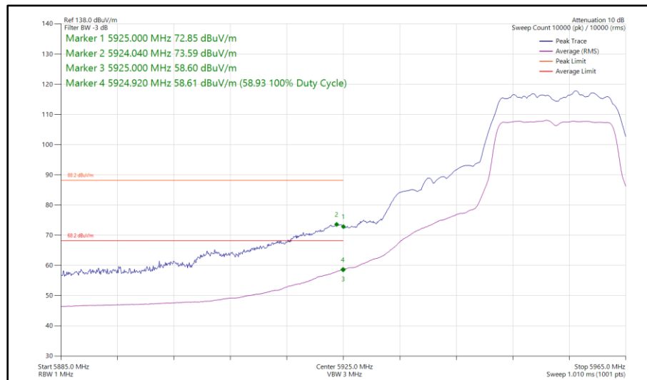
Figure 104 - 802.11a, SISO, Core 1 - 5955 MHz Band Edge Frequency 5925 MHz
