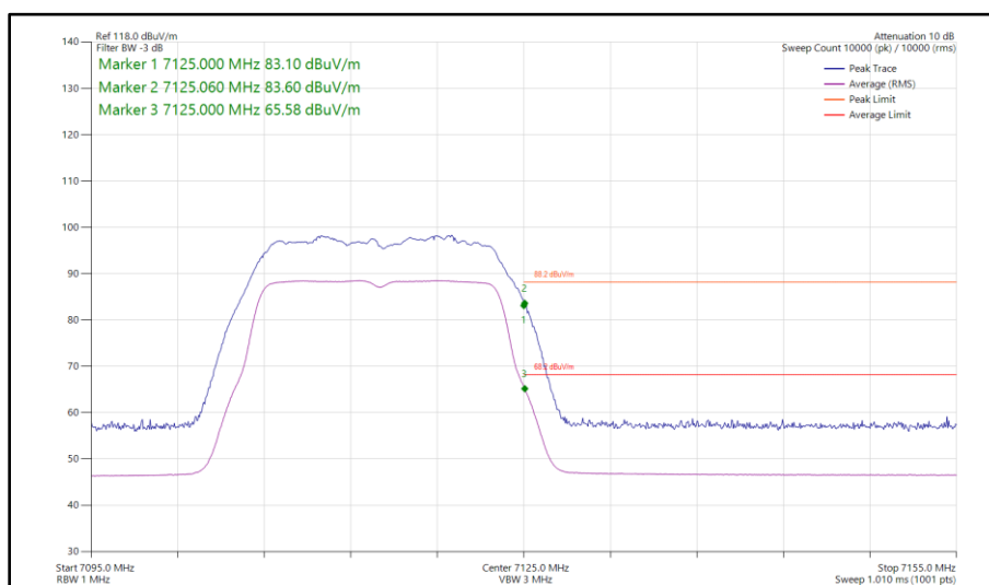
Figure 100 - 802.11a, SISO, Core 0 - 7115 MHz Band Edge Frequency 7125 MHz
