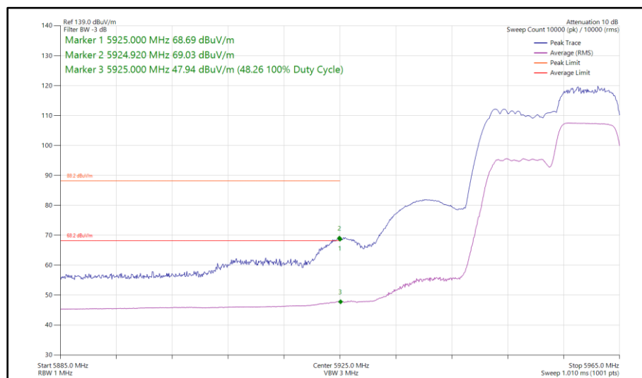
Figure 98 - 802.11ax HE20, RU 106-54, SISO, Core 0 - 5955 MHz Band Edge Frequency 5925 MHz
