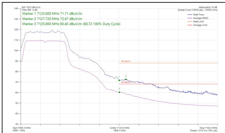
Figure 99 - 802.11a, SISO, Core 0 - 7095 MHz Band Edge Frequency 7125 MHz
