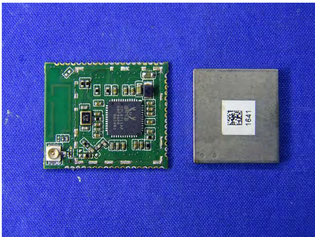
(19) EUT Photo (Module)
