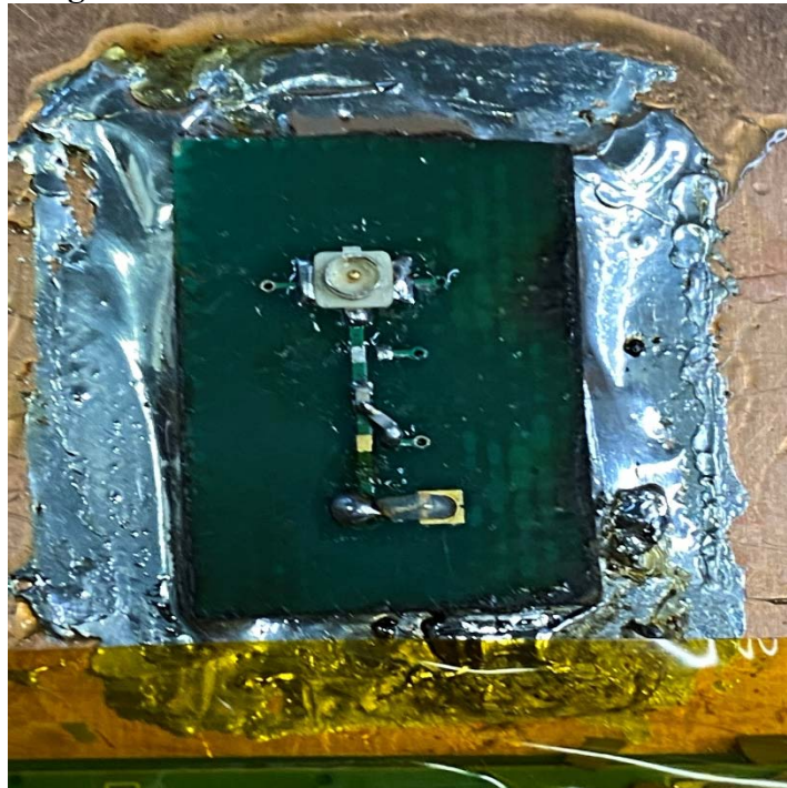
WPT Antenna Matching Soldered View
