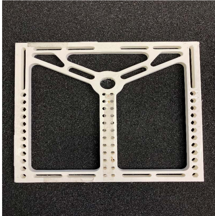
WPT Antenna Spacer View
