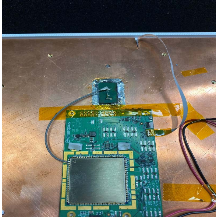
PCB Top View with Shield 2
