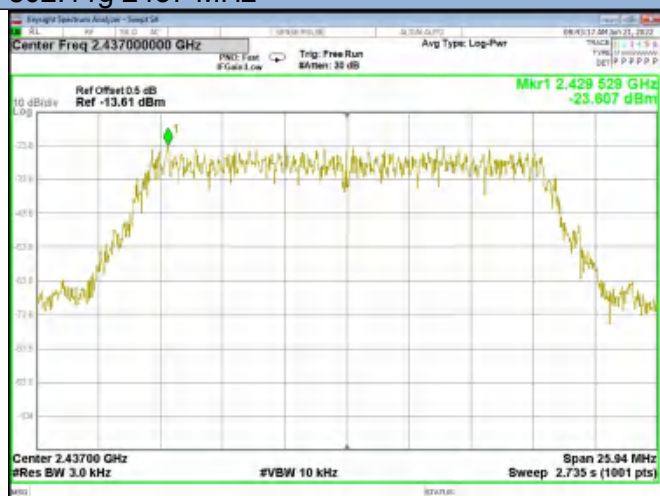
802.11g 2437 MHz
