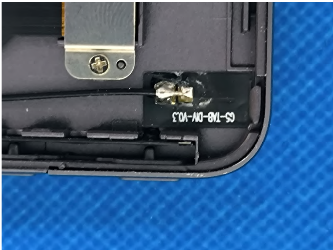
DIV Antenna
