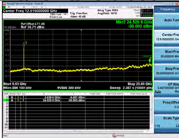
2_Spurious_Emission_2_4GWiFi_NVNT_ANT1_802_11b_2437
