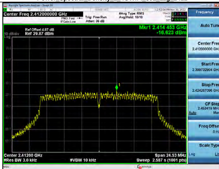
Power_Spectral_Density_2_4GWiFi_802_11g_2412
