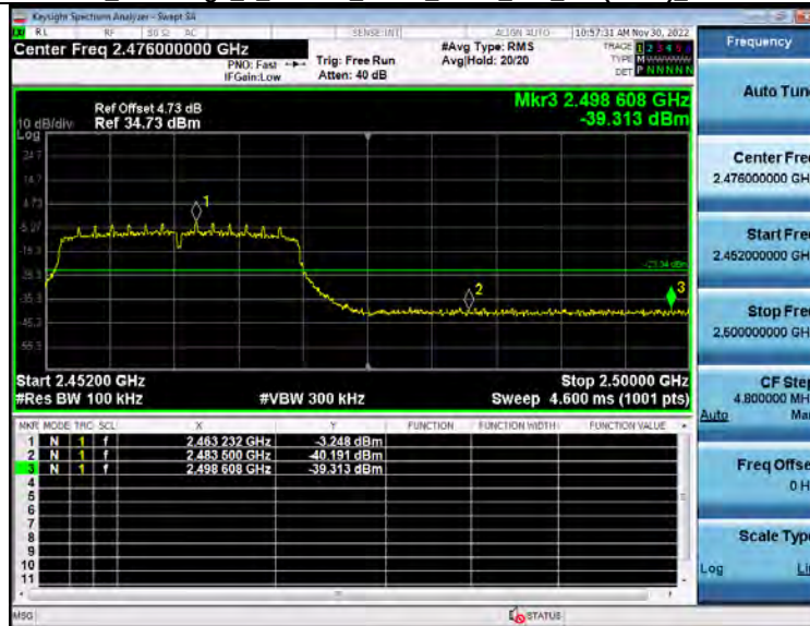
2_Bandedge 2_4GWiFi_NVNT_ANT1_802_11n(HT20)_2462
