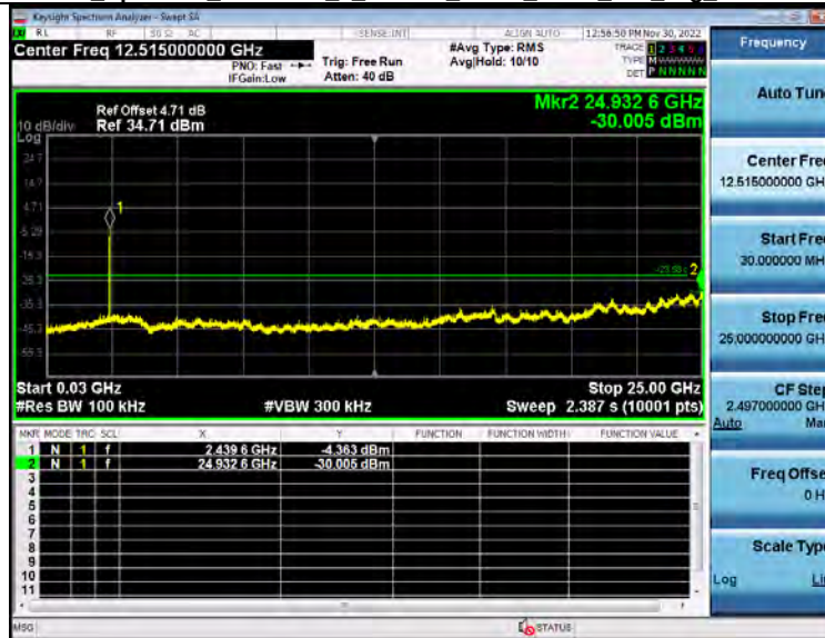
2_Spurious_Emission_2_4GWiFi_NVNT_ANT1_802_11g_2437
