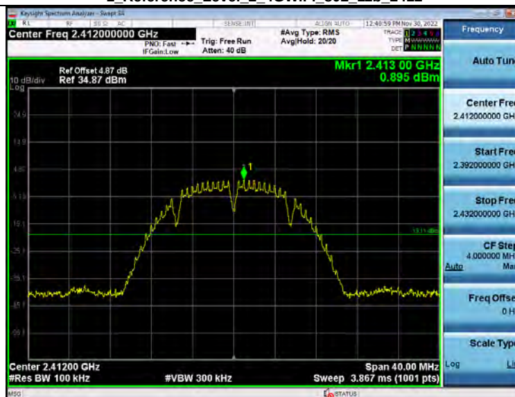
2_Bandedge 2_4GWiFi_NVNT_ANT1_802_11b_2412
