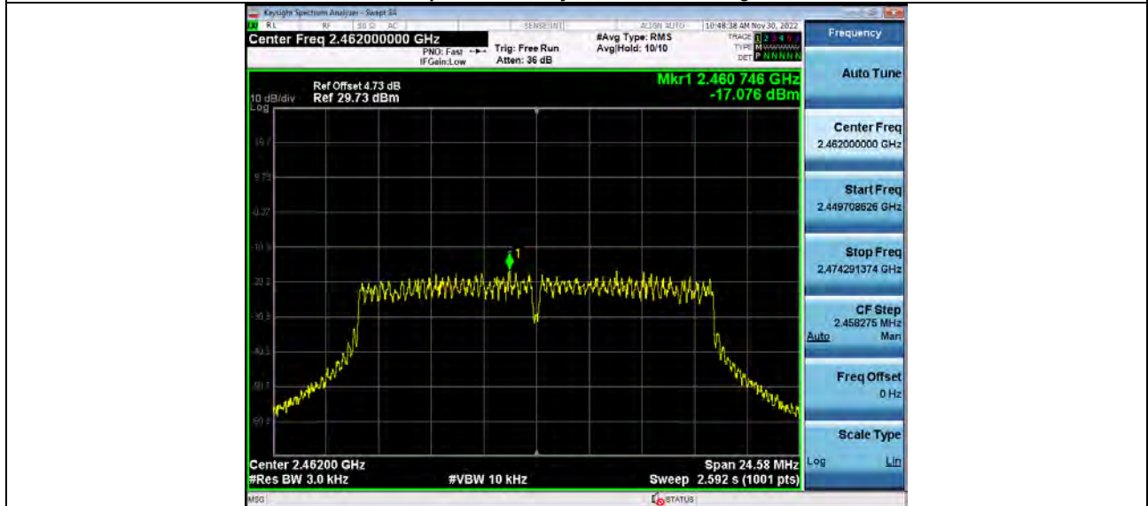
Power_Spectral_Density_2_4GWiFi_802_11g_2462
