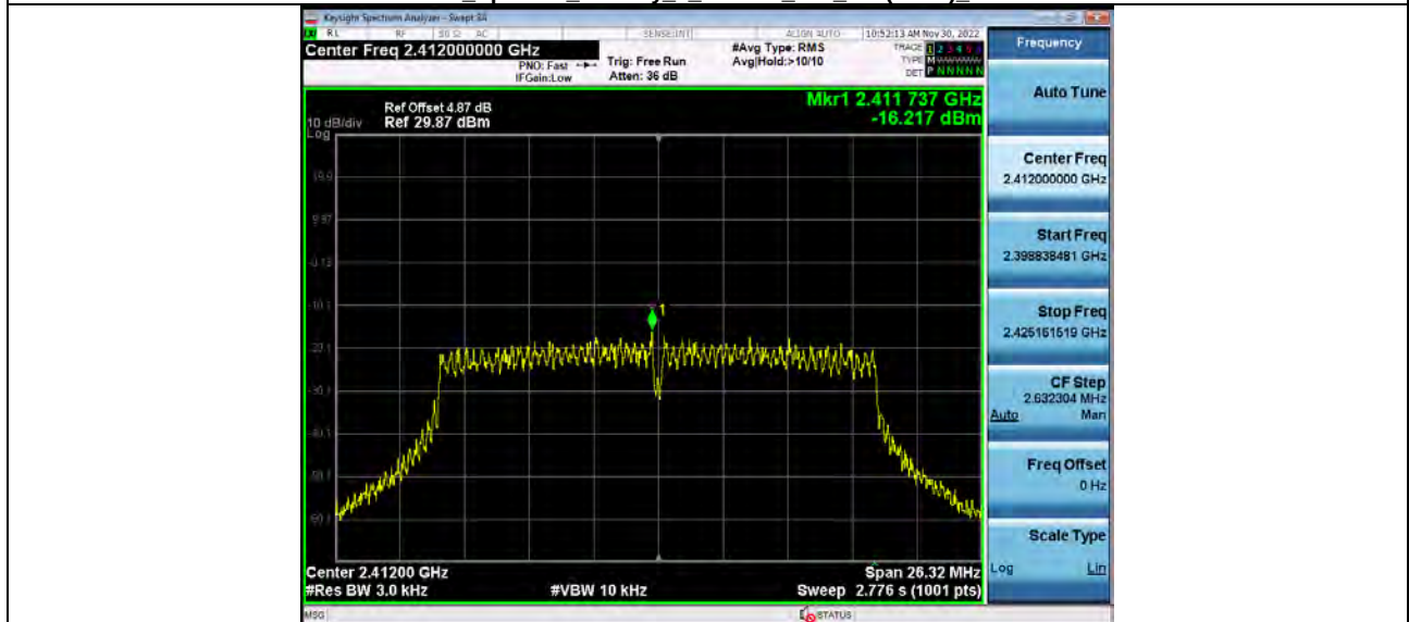
Power_Spectral_Density_2_4GWiFi_802_11n(HT20)_2412
