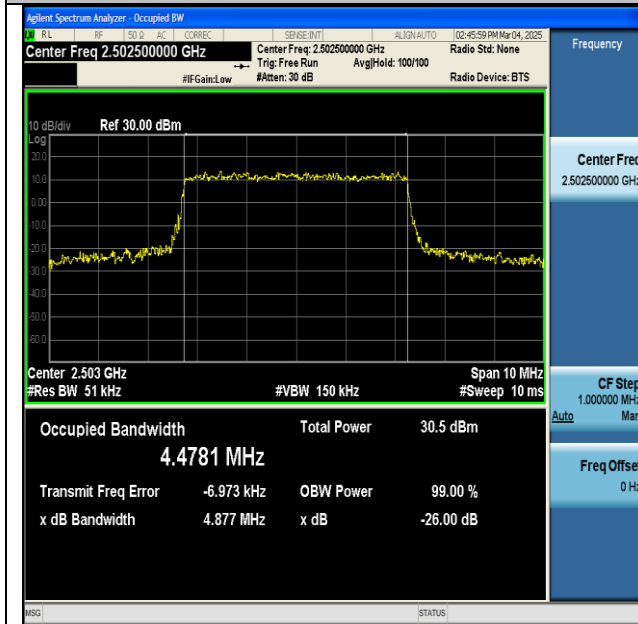
NTNV-n7-PC3-15-5-L-CP-16QAM-Outer_Full-Ant1-PASS
