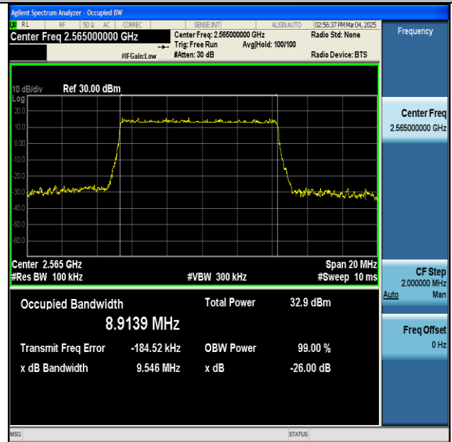
NTNV-n7-PC3-15-10-H-DFT-16QAM-Outer_Full-Ant1-PASS
