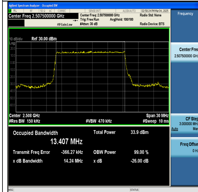
NTNV-n7-PC3-15-15-L-DFT-BPSK-Outer_Full-Ant1-PASS
