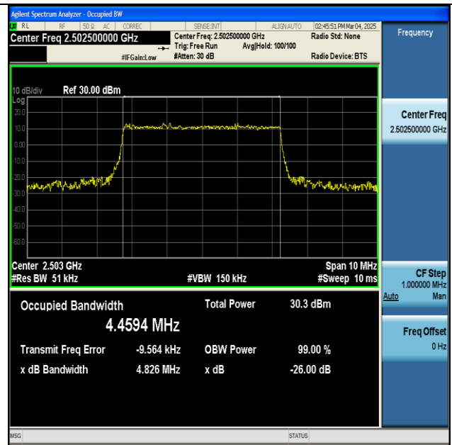
NTNV-n7-PC3-15-5-L-CP-QPSK-Outer_Full-Ant1-PASS
