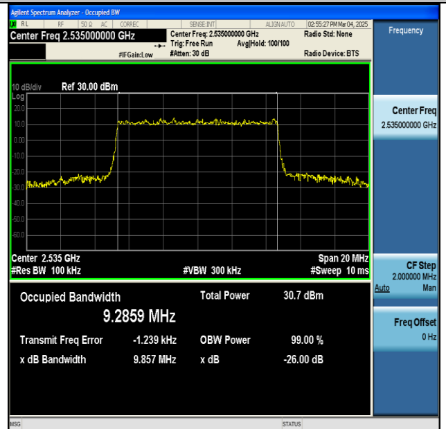
NTNV-n7-PC3-15-10-M-CP-64QAM-Outer_Full-Ant1-PASS
