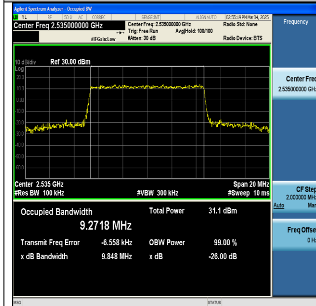
NTNV-n7-PC3-15-10-M-CP-16QAM-Outer_Full-Ant1-PASS
