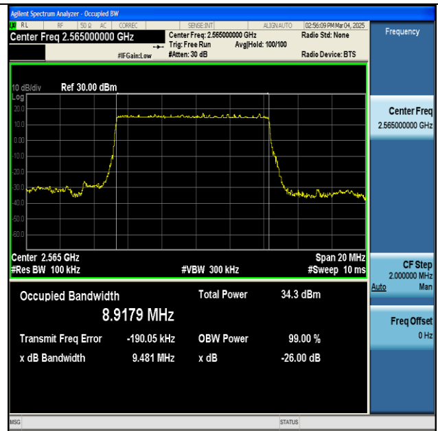
NTNV-n7-PC3-15-10-H-DFT-BPSK-Outer_Full-Ant1-PASS
