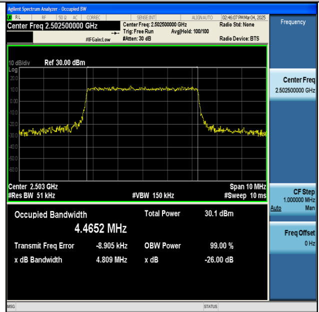
NTNV-n7-PC3-15-5-L-CP-64QAM-Outer_Full-Ant1-PASS
