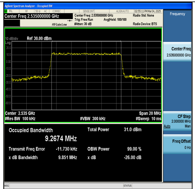
NTNV-n7-PC3-15-10-M-CP-QPSK-Outer_Full-Ant1-PASS
