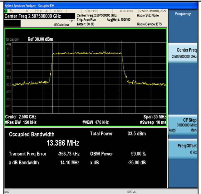
NTNV-n7-PC3-15-15-L-DFT-QPSK-Outer_Full-Ant1-PASS
