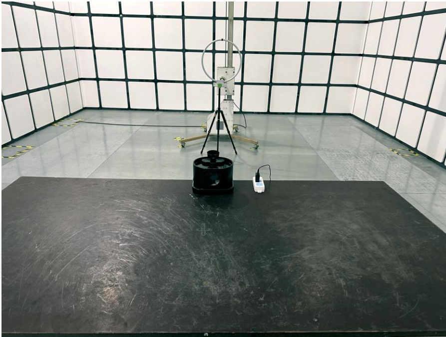
Radiated Disturbance Test (<30M)
