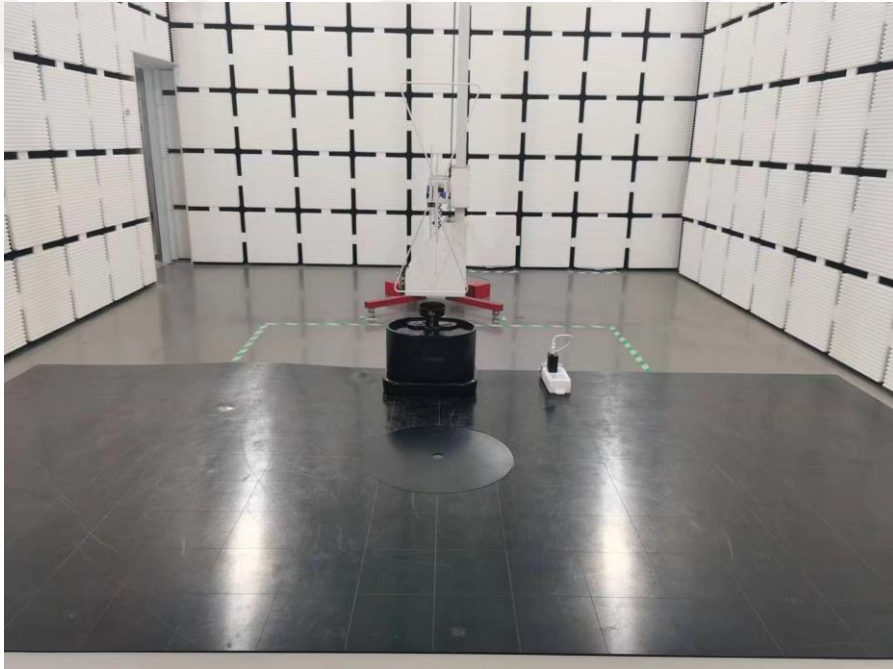
Radiated Disturbance Test (<1G)
