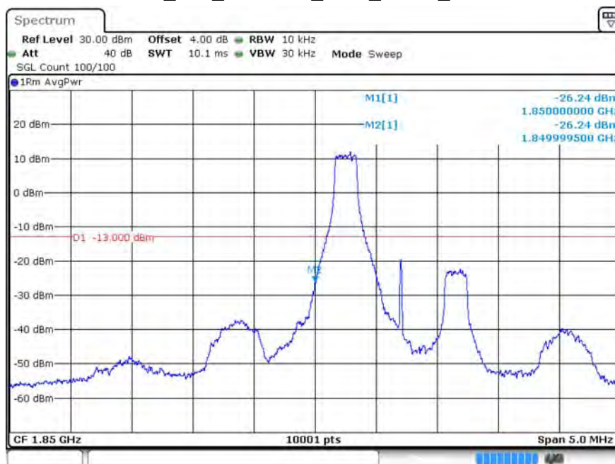
LTE_B25_CH26047_1.4M_QPSK_1RB0
