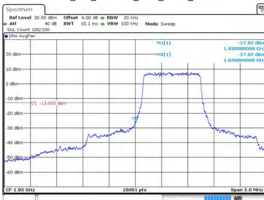
LTE_B25_CH26047_1.4M_QPSK_6RB0
