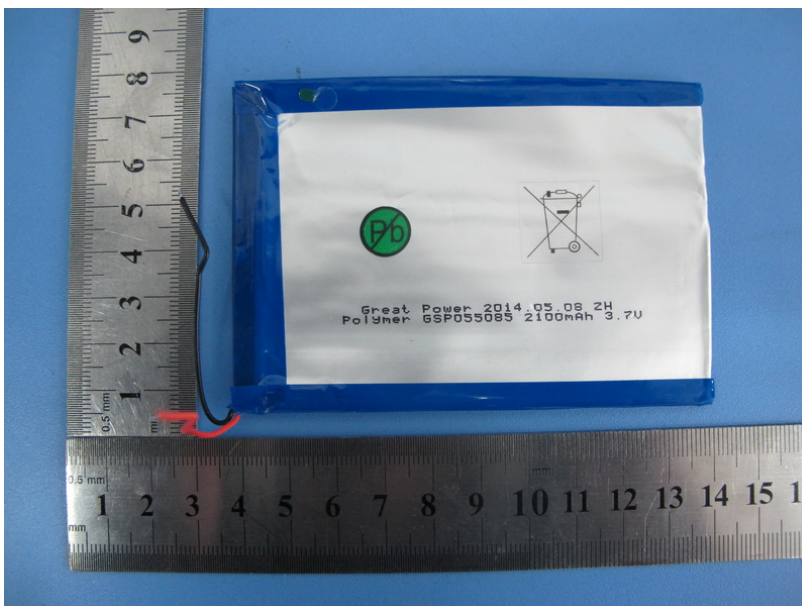
Photo 16 Appearance of Battery
