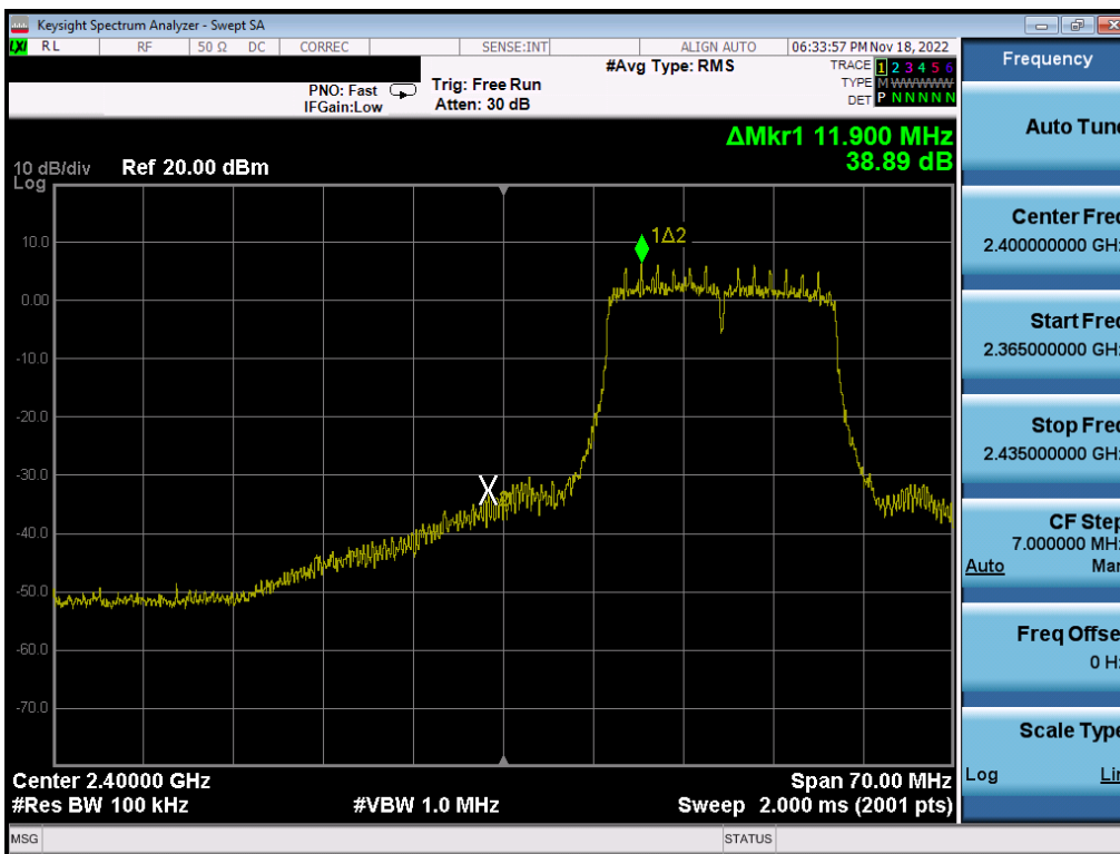
Plot 7-78. Band Edge Plot (802.11n (2.4GHz) – Ch. 2) SISO ANT 2
