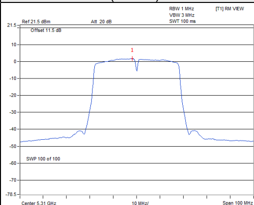
802.11ac (VHT40) / Chain 3 / CH 62
