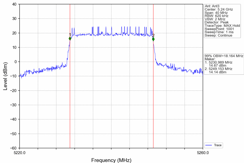
20_HCH_5240MHz_Ant3_NTNV
