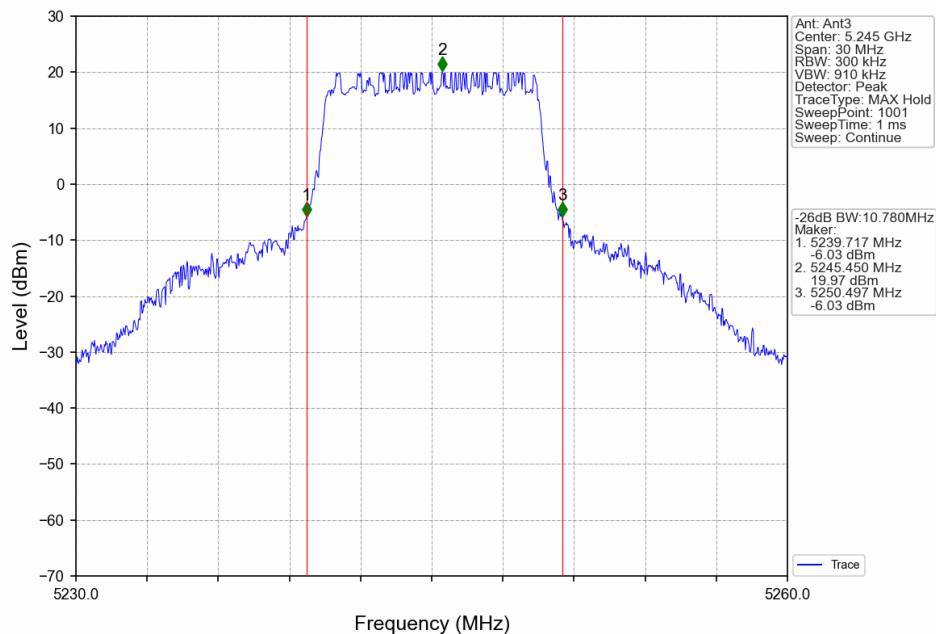
10_HCH_5245MHz_Ant3_NTNV
