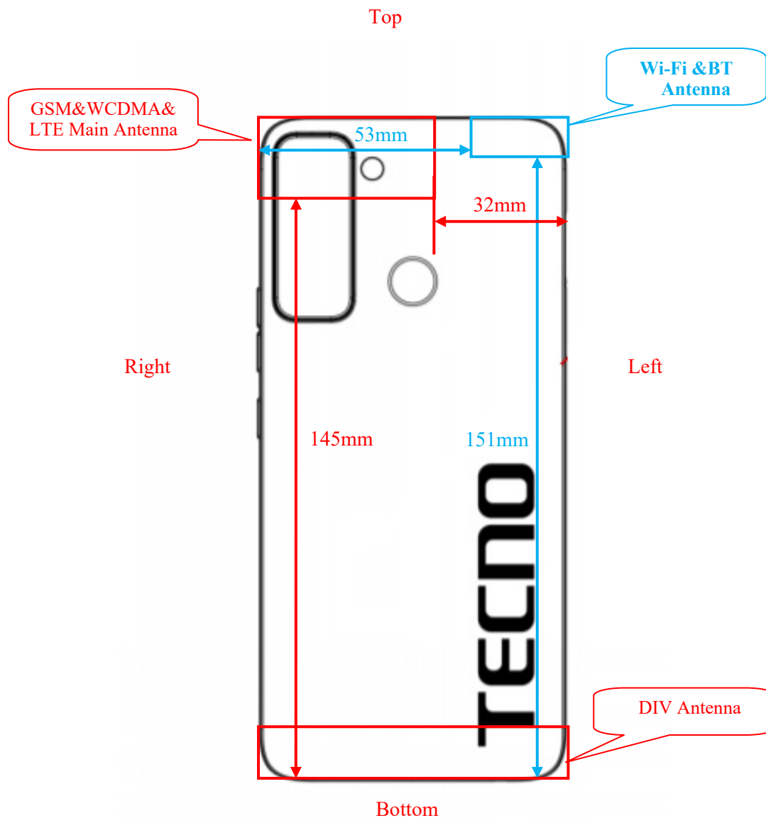
EUT Back View
