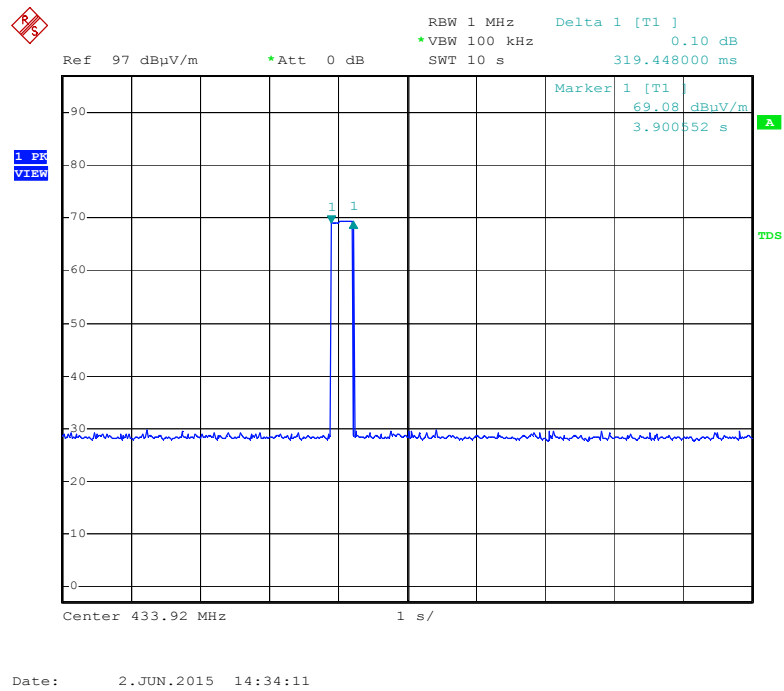
Transmitter Turn-Off Release Time, Upon Momentary Activation of Push Switch (Showing release time less than 3 second)
