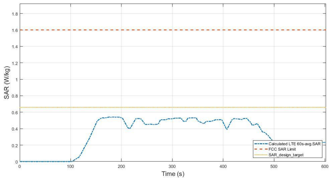
Figure 7.4-18 Total time-averaged SAR
