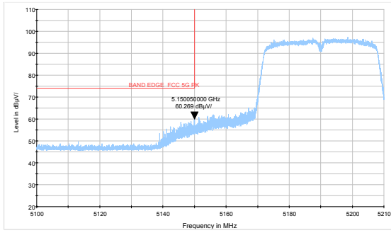
802.11ac VHT40-Channel 38: Average
