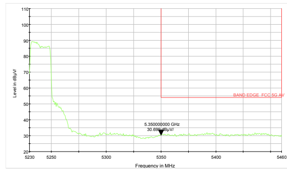
802.11ac VHT20 -Channel 48: Average
