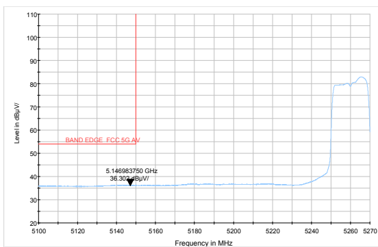
802.11ac VHT20-Channel 52: Average
