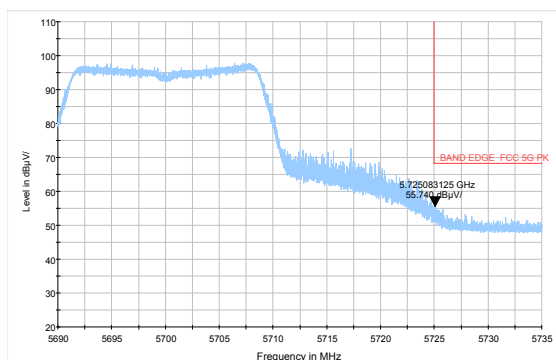
802.11ac VHT20 -Channel 140: Peak
