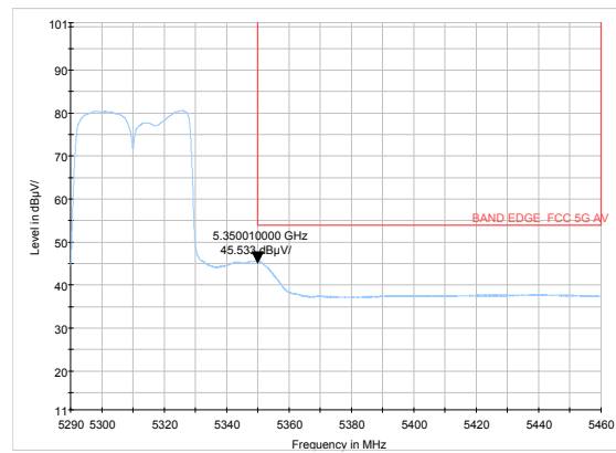
802.11ac VHT40-Channel 62: Average
