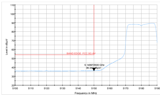
802.11ac VHT20-Channel 36: Average
