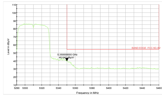
802.11ac VHT40-Channel 62: Average
