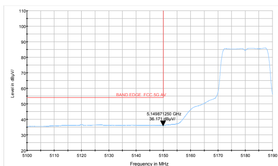
802.11a-Channel 36: Average
