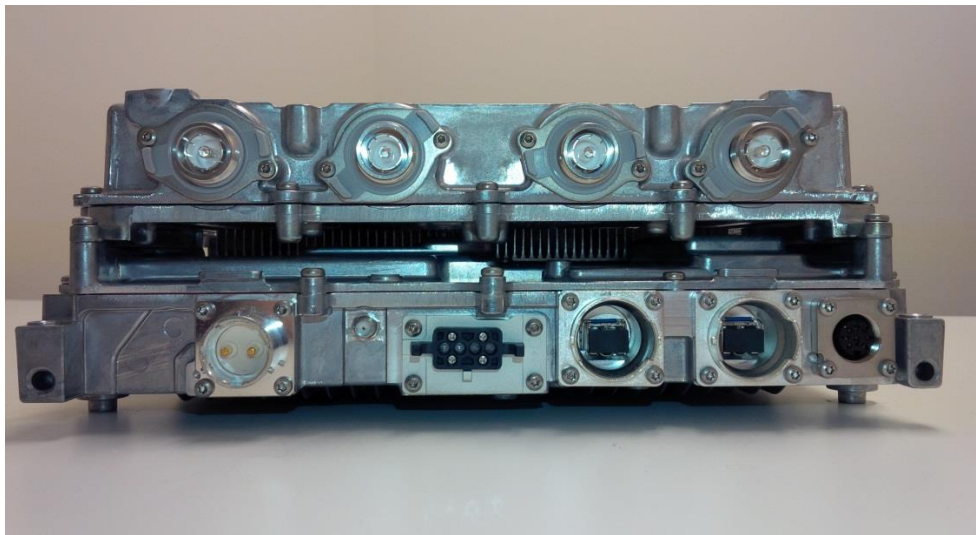
Figure 4: RRUS 32A B66A Front View
