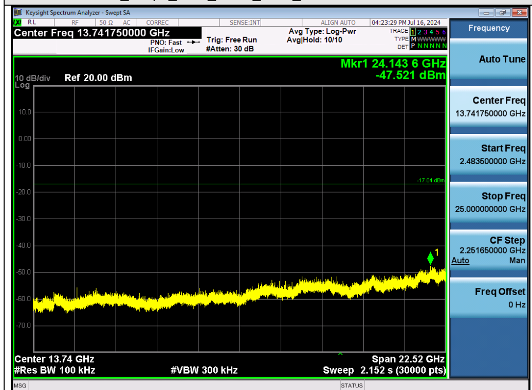
Test_Graph_2.4G_ANT1_2441_Higher Band Emissions
