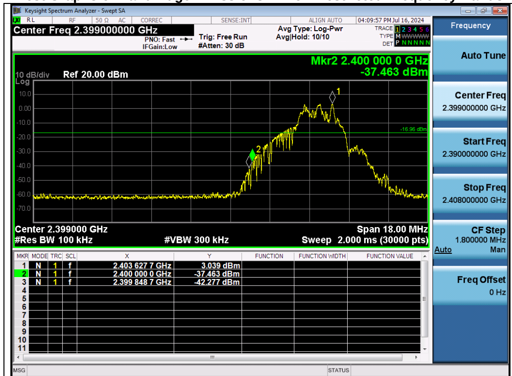
Test_Graph_2.4G_ANT1_2403_Lower Band Edge Emissions
