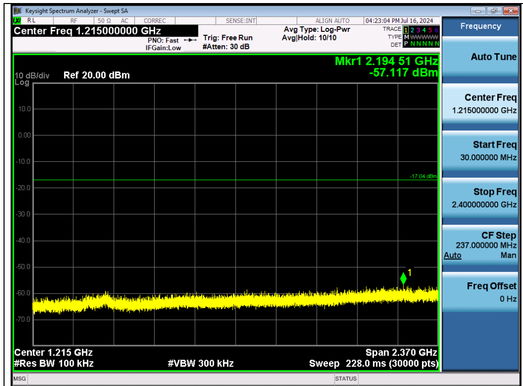
Test_Graph_2.4G_ANT1_2441_Lower Band Emissions
