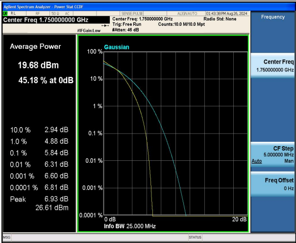
Band4-10MHz-16QAM-20350-50RB#0-PASS
