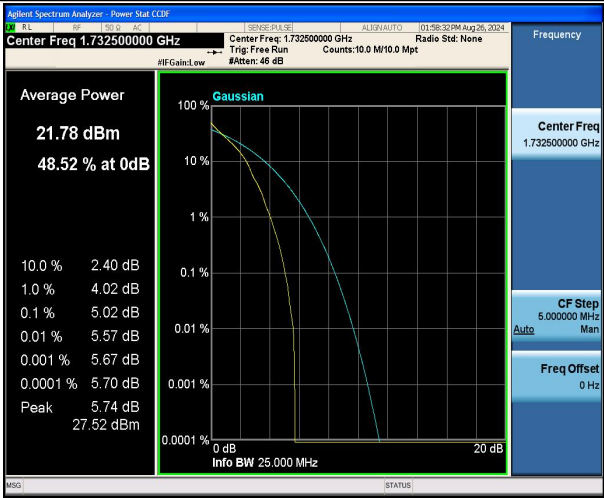
Band4-15MHz-QPSK-20175-1RB#0-PASS
