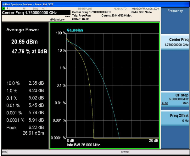
Band4-10MHz-QPSK-20350-50RB#0-PASS
