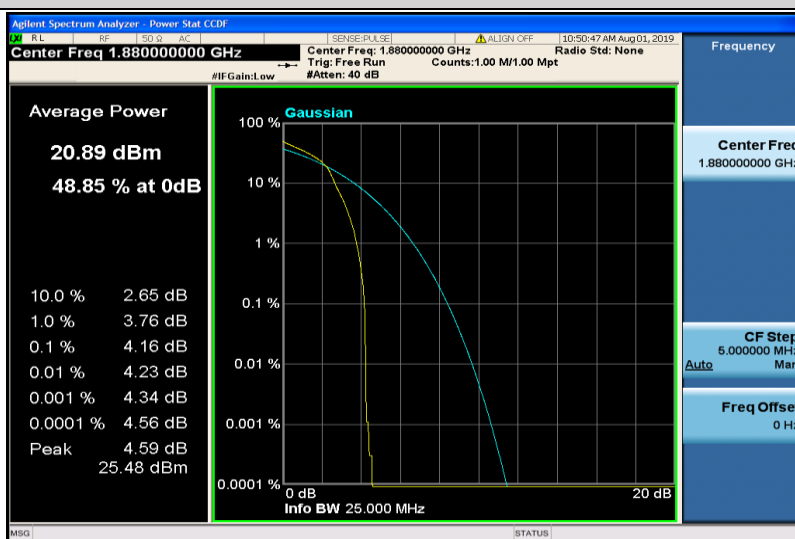
Band2-15MHz-16QAM-18900-1RB#0
