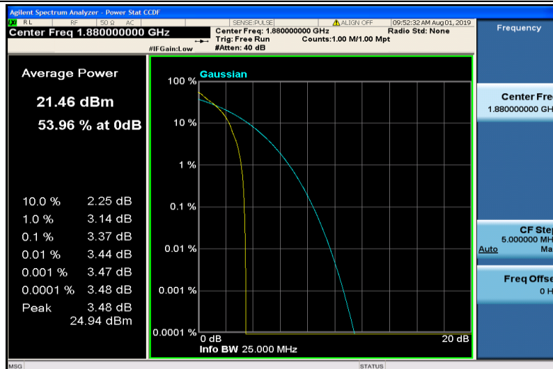
Band2-1.4MHz-QPSK-18900-1RB#0
