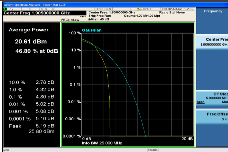
Band2-10MHz-16QAM-19150-1RB#0
