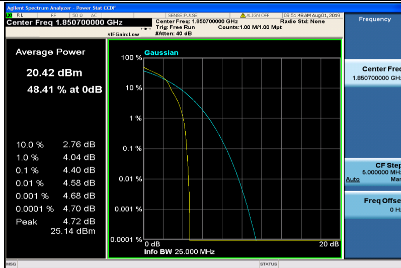
Band2-1.4MHz-16QAM-18607-1RB#0
