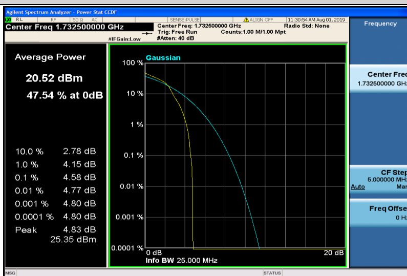
Band4-1.4MHz-16QAM-20175-1RB#0
