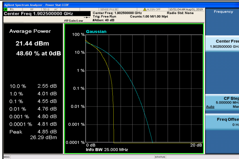
Band2-15MHz-QPSK-19125-1RB#0
