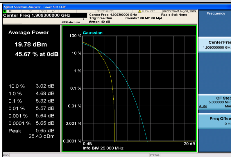
Band2-1.4MHz-16QAM-19193-6RB#0
