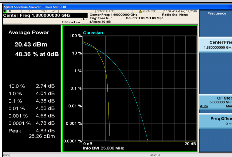
Band2-10MHz-16QAM-18900-1RB#0
