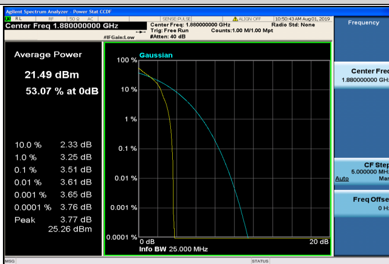
Band2-15MHz-QPSK-18900-1RB#0
