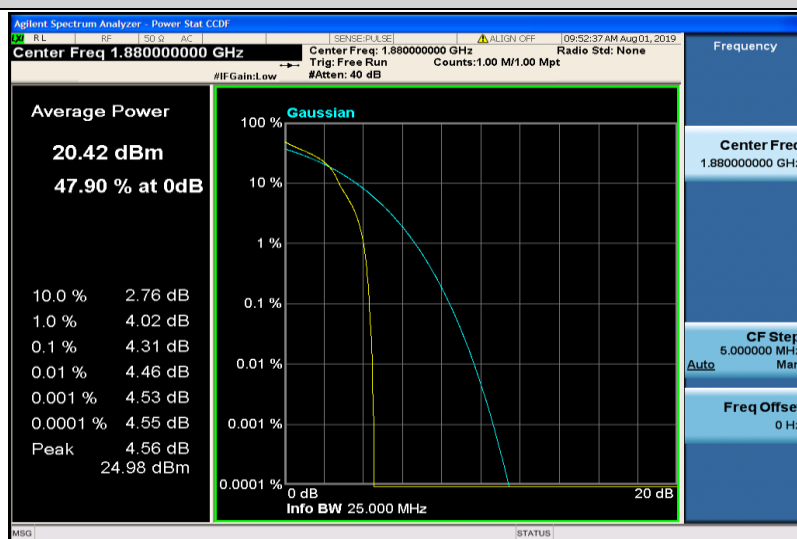
Band2-1.4MHz-16QAM-18900-1RB#0
