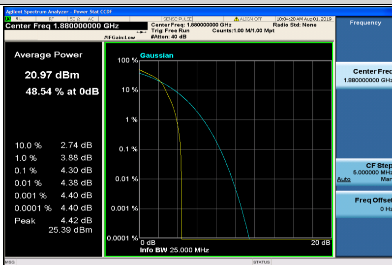
Band2-3MHz-16QAM-18900-1RB#0
