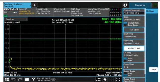
Band13-5MHz-QPSK-23255-1RB#24-0.15~30-PASS
