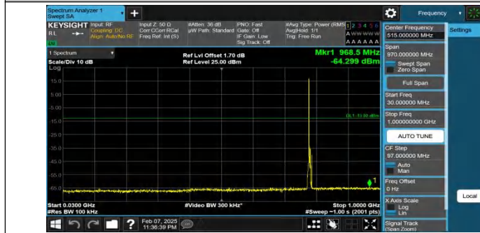
Band13-5MHz-QPSK-23255-1RB#0-30~1000-PASS
