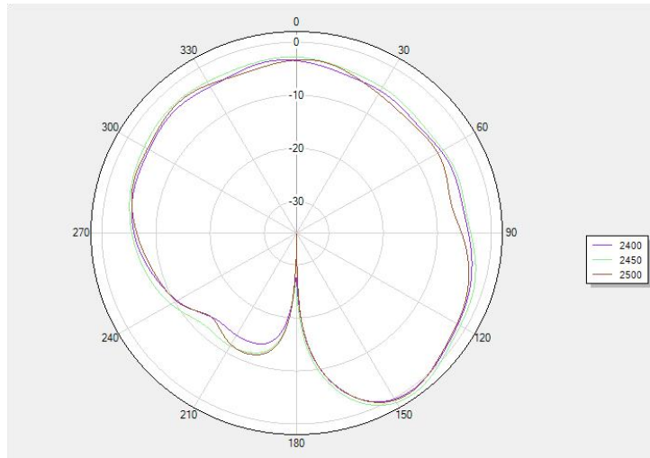
Phi 90 2D
