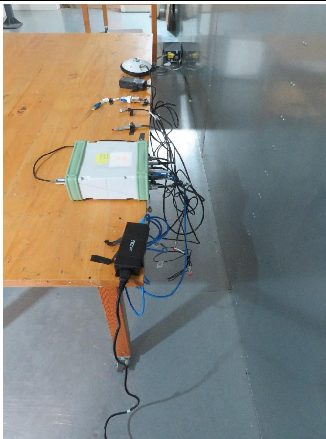
Setup for measurements 150 kHz – 30 MHz (with PoE)
