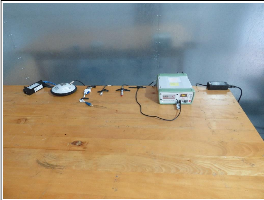
Setup for measurements 150 kHz – 30 MHz (with AC/DC Adapter)
