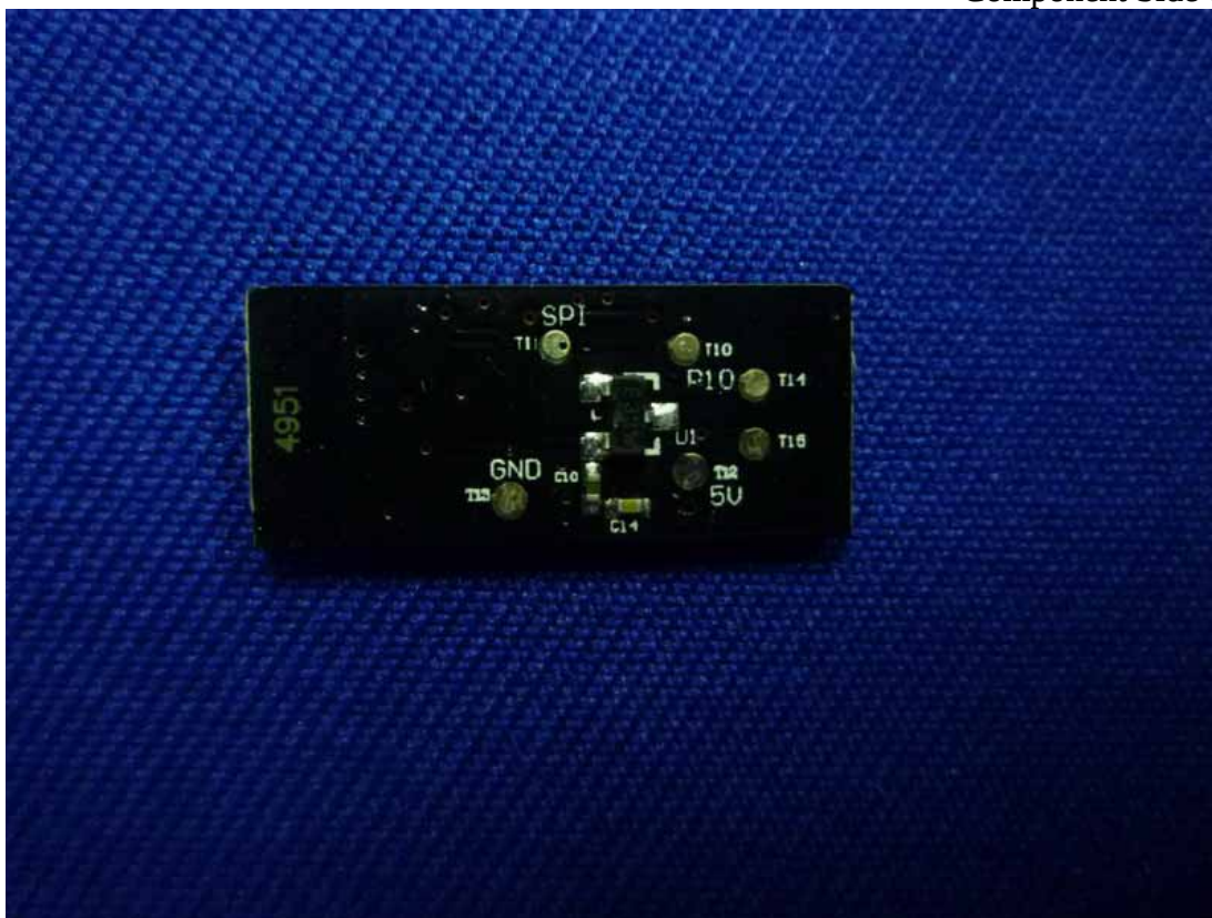
Figure 6 Component Side of the PCB
