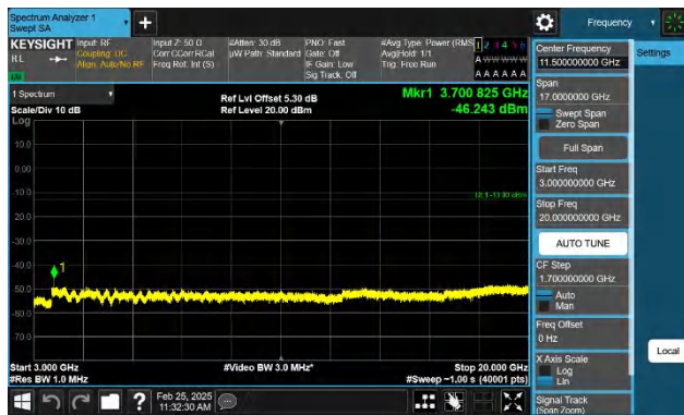
Band2-10MHz-QPSK-18650-1RB#0-3000~20000-PASS
