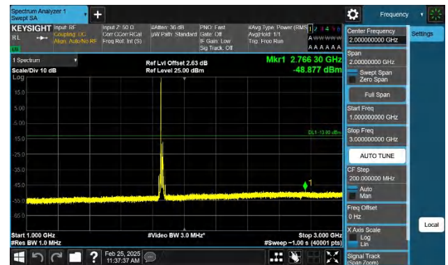
Band2-15MHz-QPSK-18675-1RB#0-1000~3000-PASS
