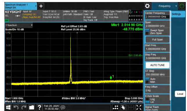
Band2-10MHz-QPSK-19150-1RB#0-1000~3000-PASS
