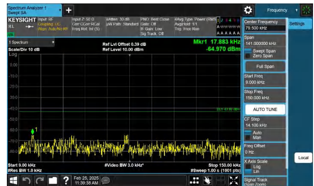
Band2-15MHz-QPSK-18900-1RB#74-0.009~0.15-PASS
