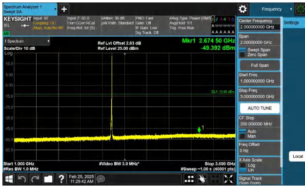
Band2-5MHz-QPSK-18900-1RB#24-1000~3000-PASS
