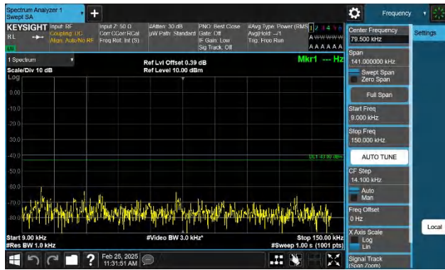
Band2-10MHz-QPSK-18650-1RB#0-0.009~0.15-PASS
