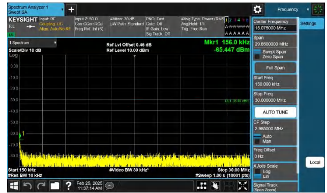
Band2-15MHz-QPSK-18675-1RB#0-0.15~30-PASS
