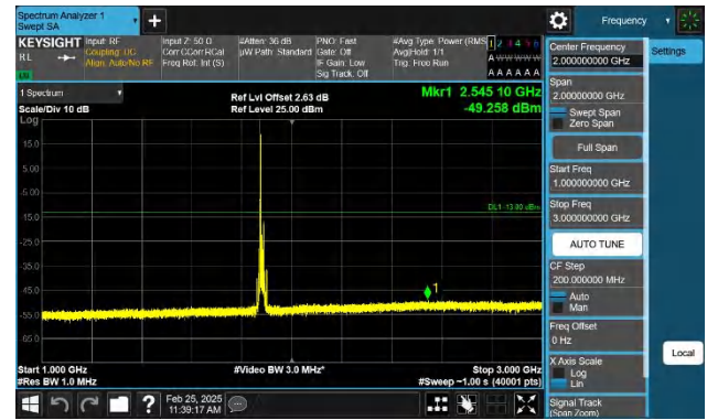
Band2-15MHz-QPSK-18900-1RB#0-1000~3000-PASS
