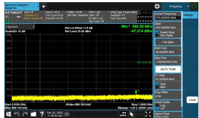
Band2-15MHz-QPSK-18900-1RB#74-30~1000-PASS
