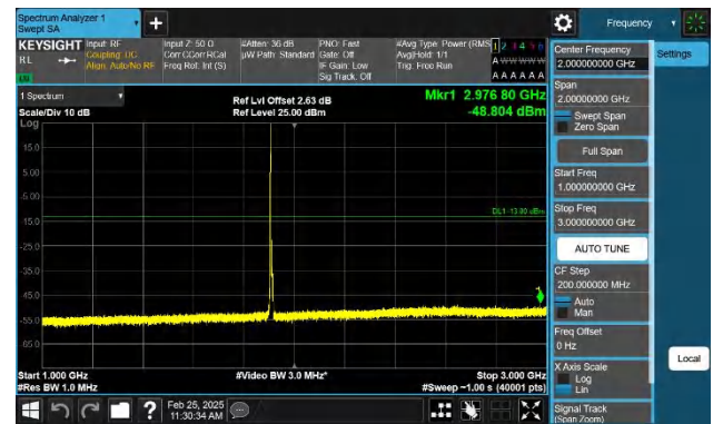
Band2-5MHz-QPSK-19175-1RB#0-1000~3000-PASS
