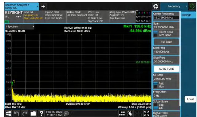
Band2-5MHz-QPSK-18900-1RB#0-0.15~30-PASS
