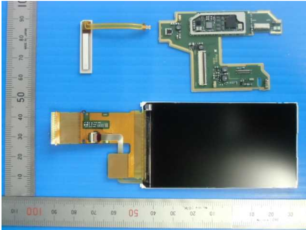
LCD PCB
