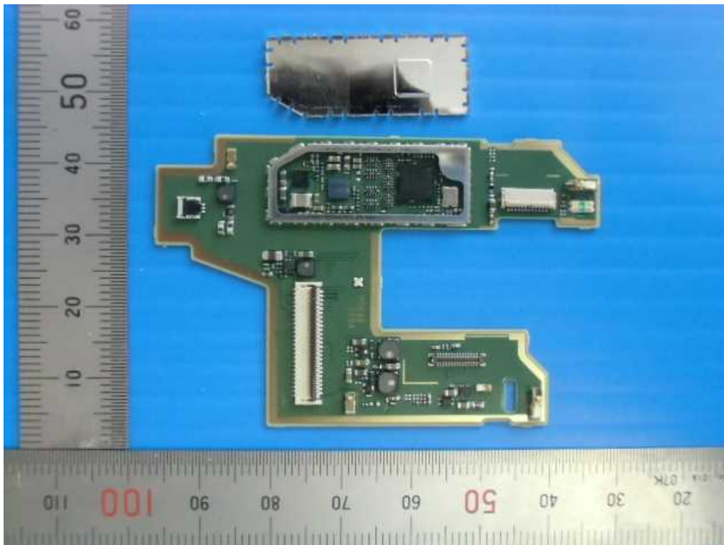
LCD PCB
