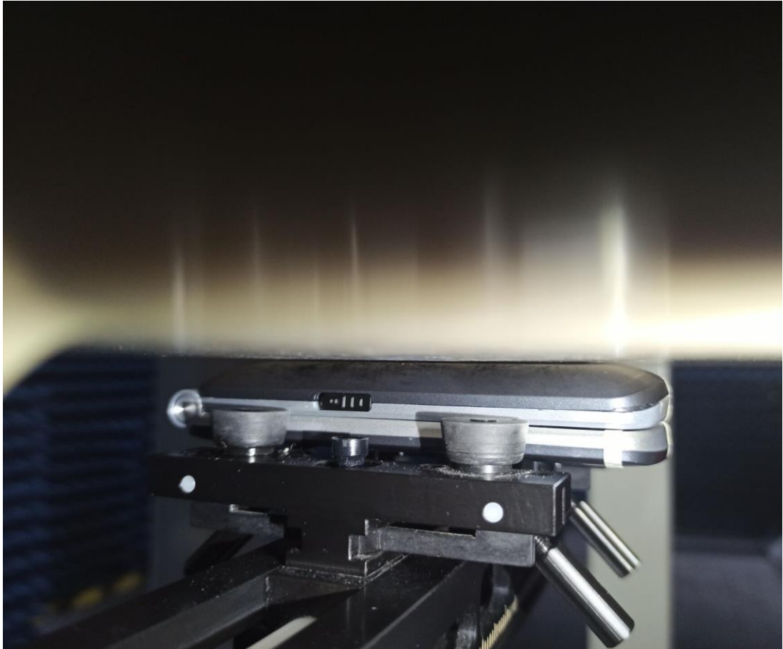
DUT with device holder (DUT direct contact with the phantom)
