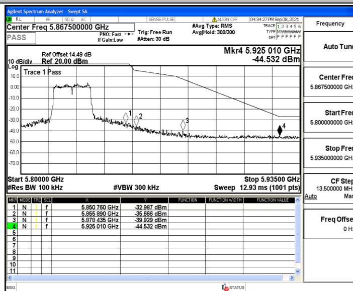
11AC20MIMO_Ant2_High_5825
