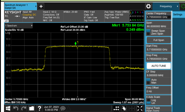
802.11ax-HE80 Power Spectral Density - Ant 1
