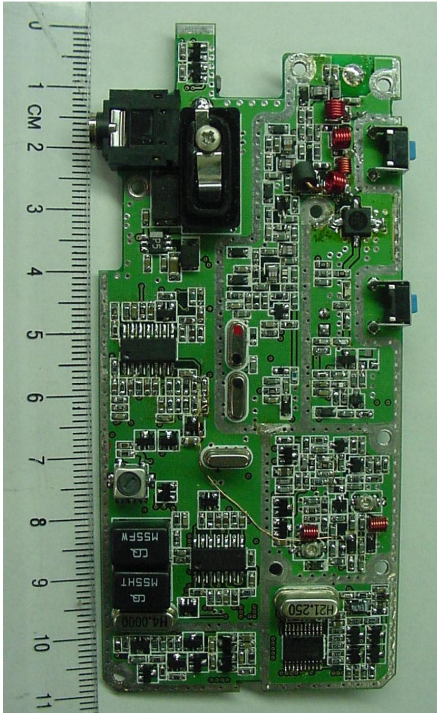
PHOTOGRAPH 5: FRONT VIEW OF PCB BOARD
