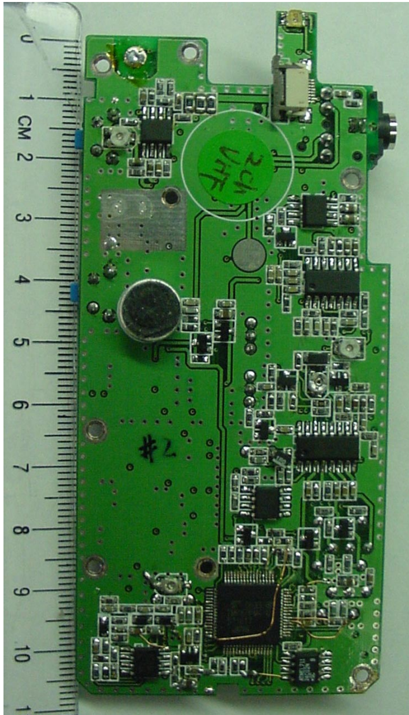
PHOTOGRAPH 6: REAR VIEW OF PCB BOARD
