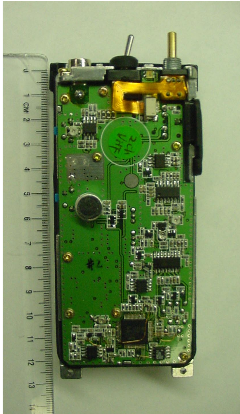
PHOTOGRAPH 7: PCB IN CHASSIS
