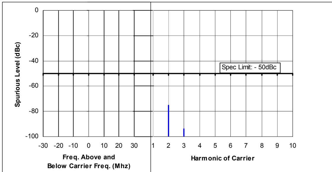
Figure 6F-4: 5.8 Watts, 136.0125 MHz, 25 KHz Channel Spacing
