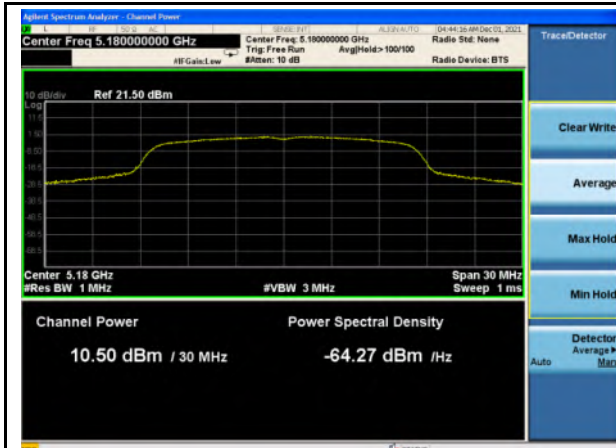
Output Power_U-NII-1_802.11a_5180
