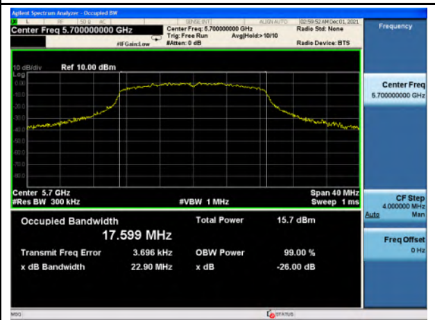
26 dB & 99% BW_U-NII-2C_802.11n_5700
