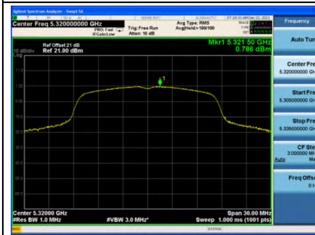
PSD_U-NII-2A_802.11a_5320
