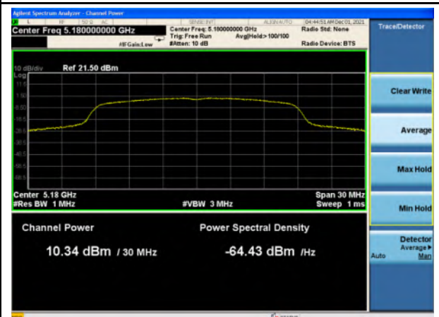
Output Power_U-NII-1_802.11n_5180
