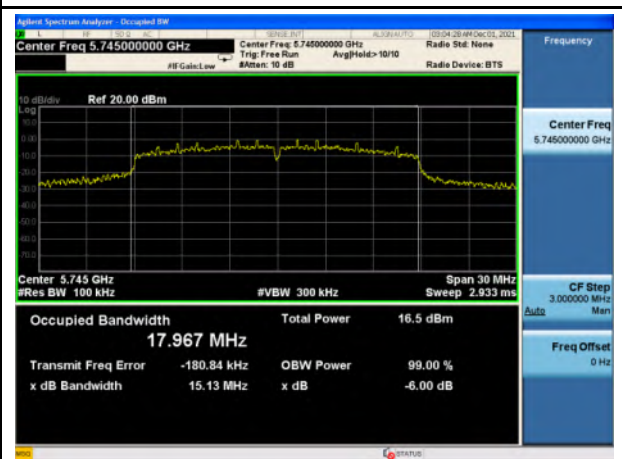
6 dB & 99% BW_U-NII-3_802.11n_5745
