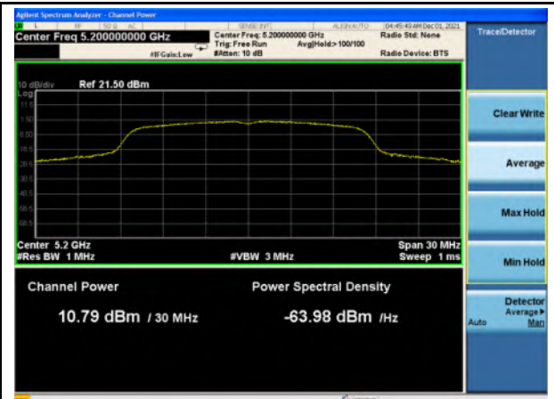
Output Power_U-NII-1_802.11a_5200
