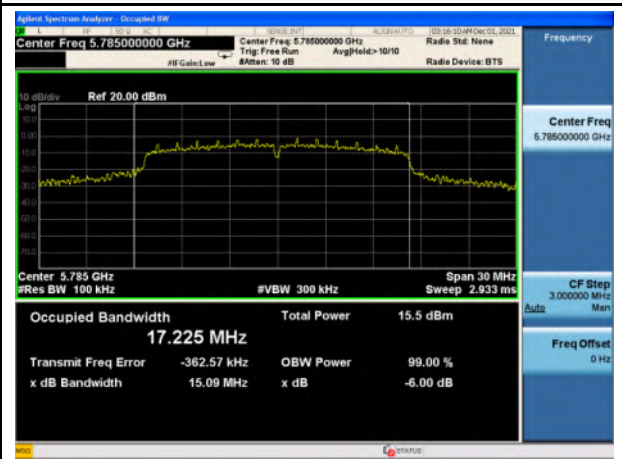
6 dB & 99% BW_U-NII-3_802.11a_5785
