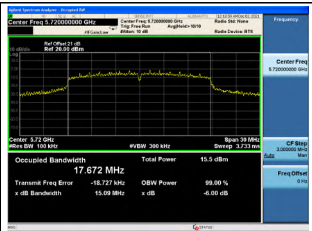
6 dB & 99% BW_U-NII-3_802.11a_5720
