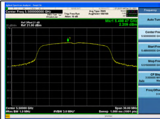
PSD_U-NII-2C_802.11a_5500
