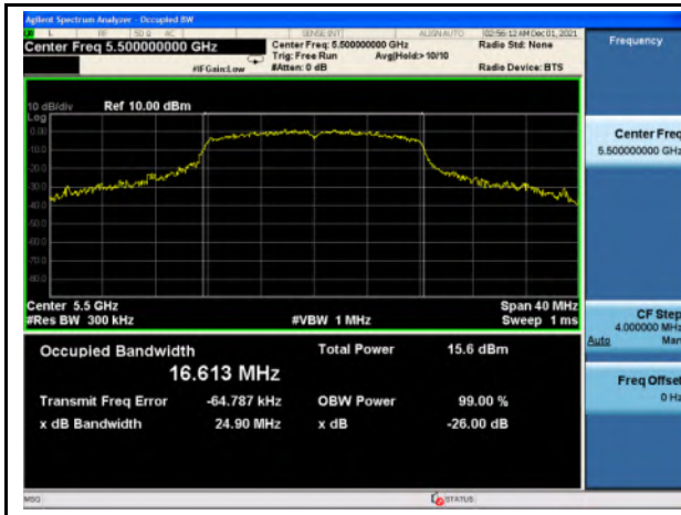
26 dB & 99% BW_U-NII-2C_802.11a_5500
