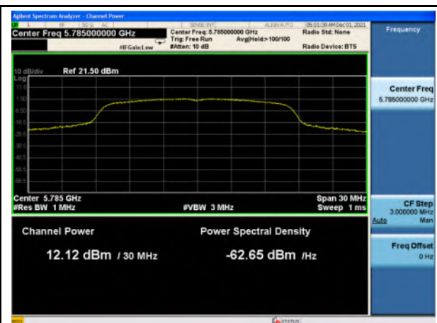
Output Power_U-NII-3_802.11a_5785
