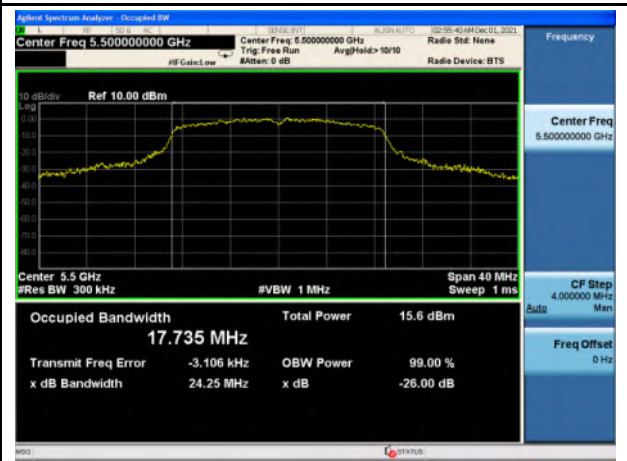
26 dB & 99% BW_U-NII-2C_802.11n_5500
