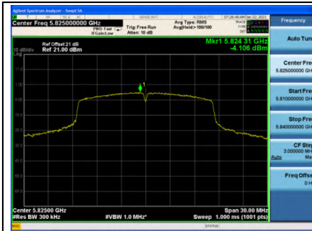
PSD_U-NII-3_802.11a_5825
