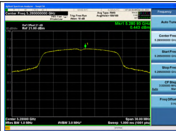
PSD_U-NII-2A_802.11a_5280
