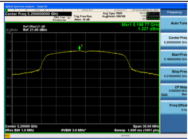
PSD_U-NII-1_802.11a_5200
