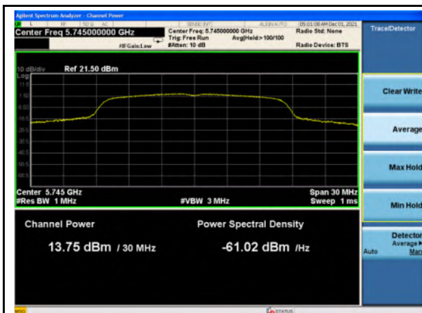
Output Power_U-NII-3_802.11a_5745
