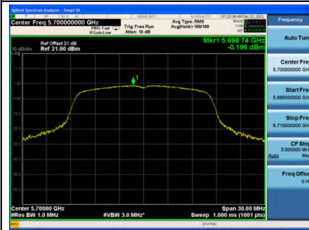
PSD_U-NII-2C_802.11a_5700
