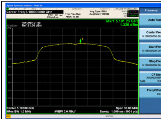
PSD_U-NII-1_802.11a_5180
