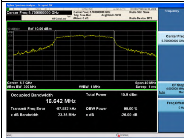
26 dB & 99% BW_U-NII-2C_802.11a_5700
