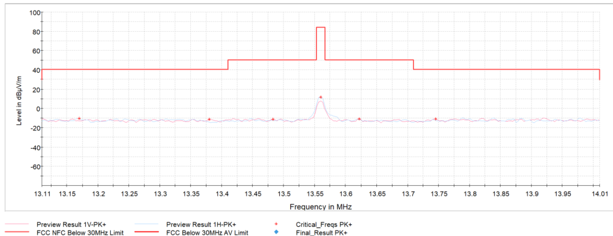
Plot 7-6. In Band Radiated Spurious Emissions (CE B 848kbps, with AC/DC Adapter and Magnetic Charger)
