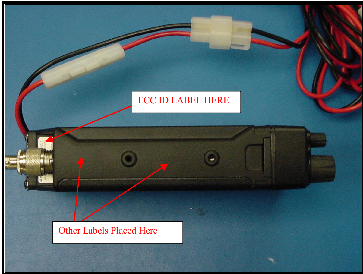
PHOTOGRAPH 1: LABEL LOCATIONS
