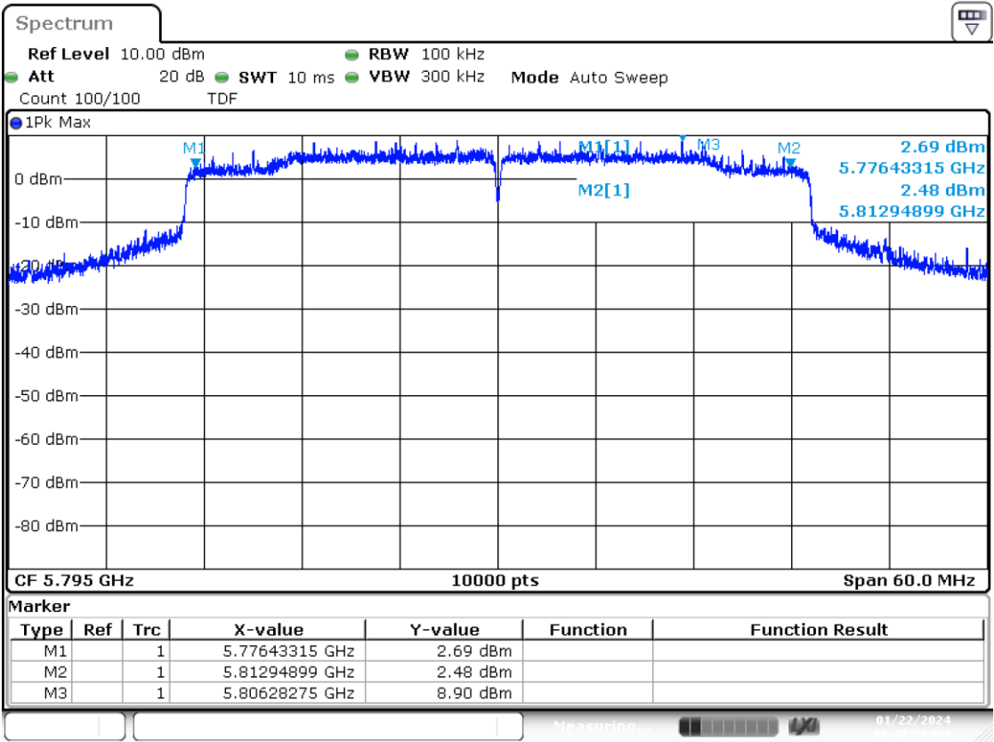
SISO B-802.11ax/be40-CH159-MCS0
