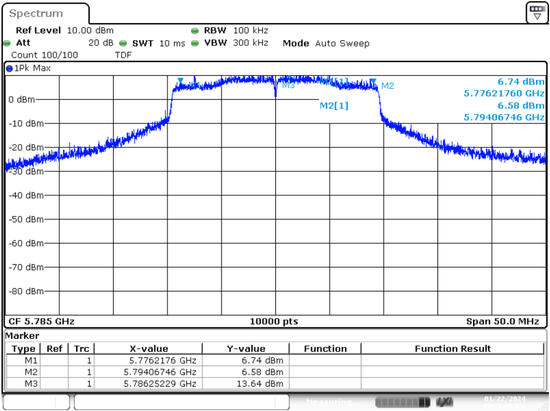
SISO B-802.11ax/be20-CH157-MCS0
