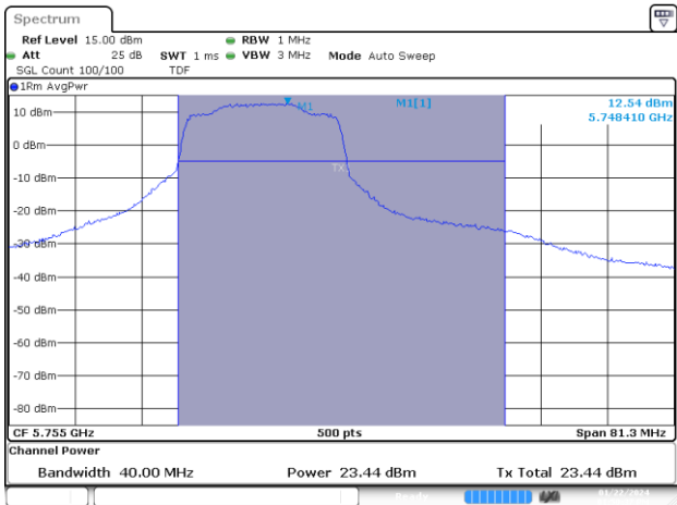
MIMO B-802.11ax/be40-CH151-MCS0 20m
