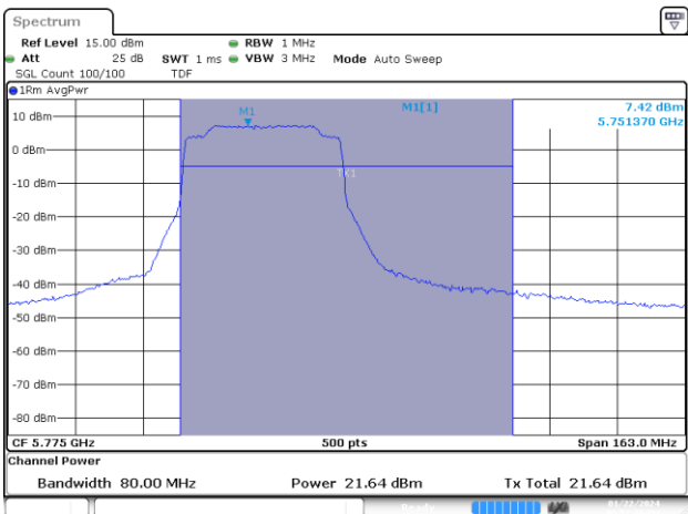
MIMO B-802.11ax/be80-CH155-MCS0 40m
