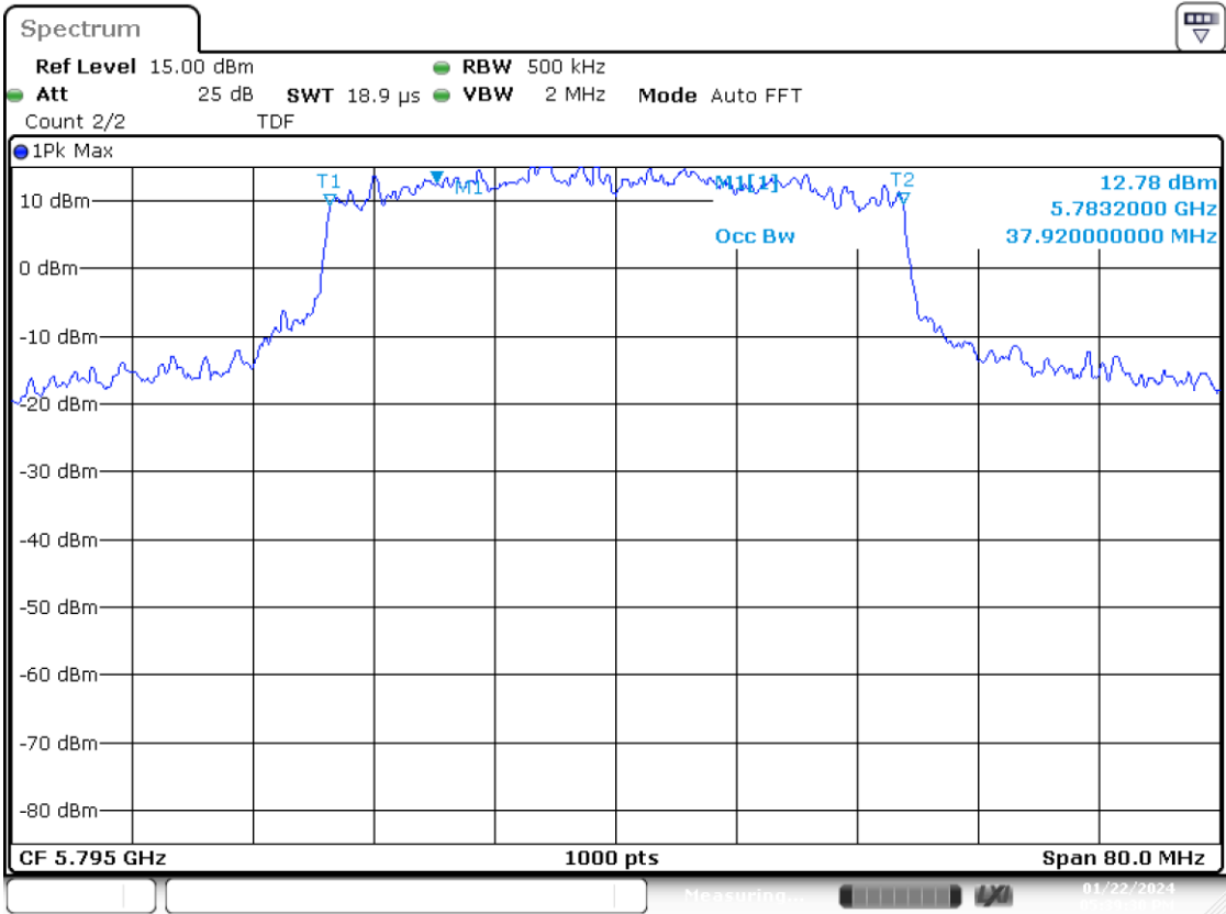
SISO B-802.11ax/be40-CH159-MCS0
