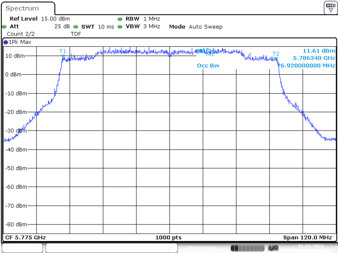
MIMO A-802.11ax/be80-CH155-MCS0
