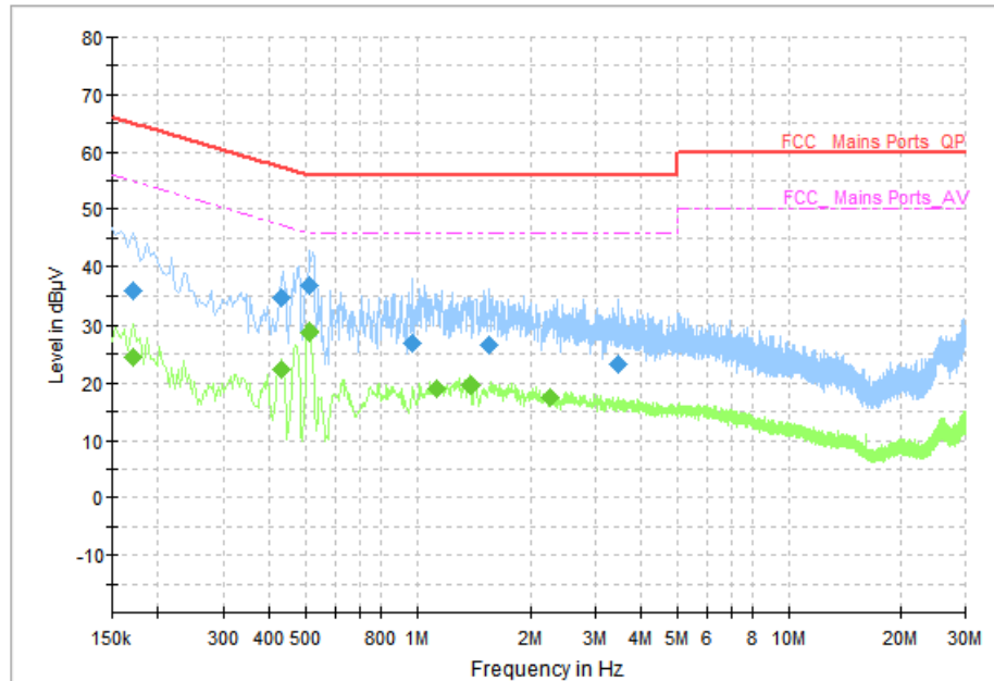
Fig. 84 AC Powerline Conducted Emission (Traffic, AE3, 120V)
