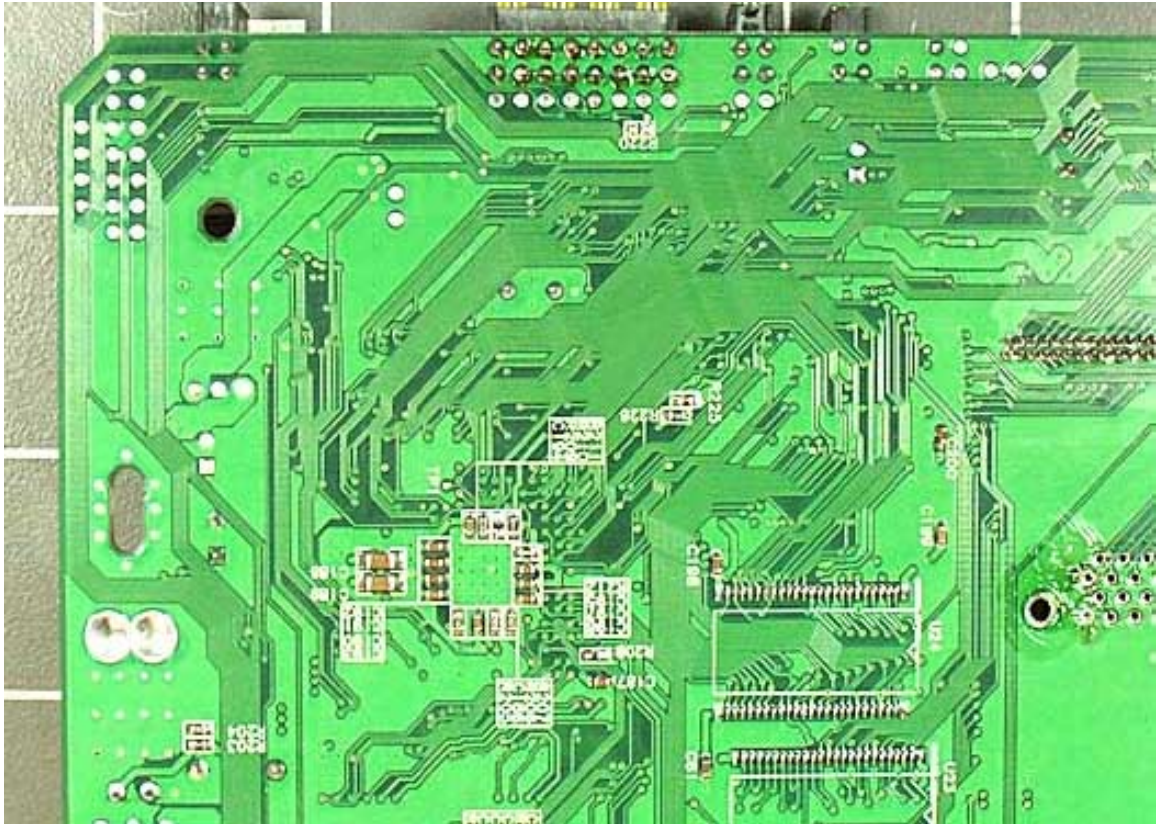
PCB Bottom #3
