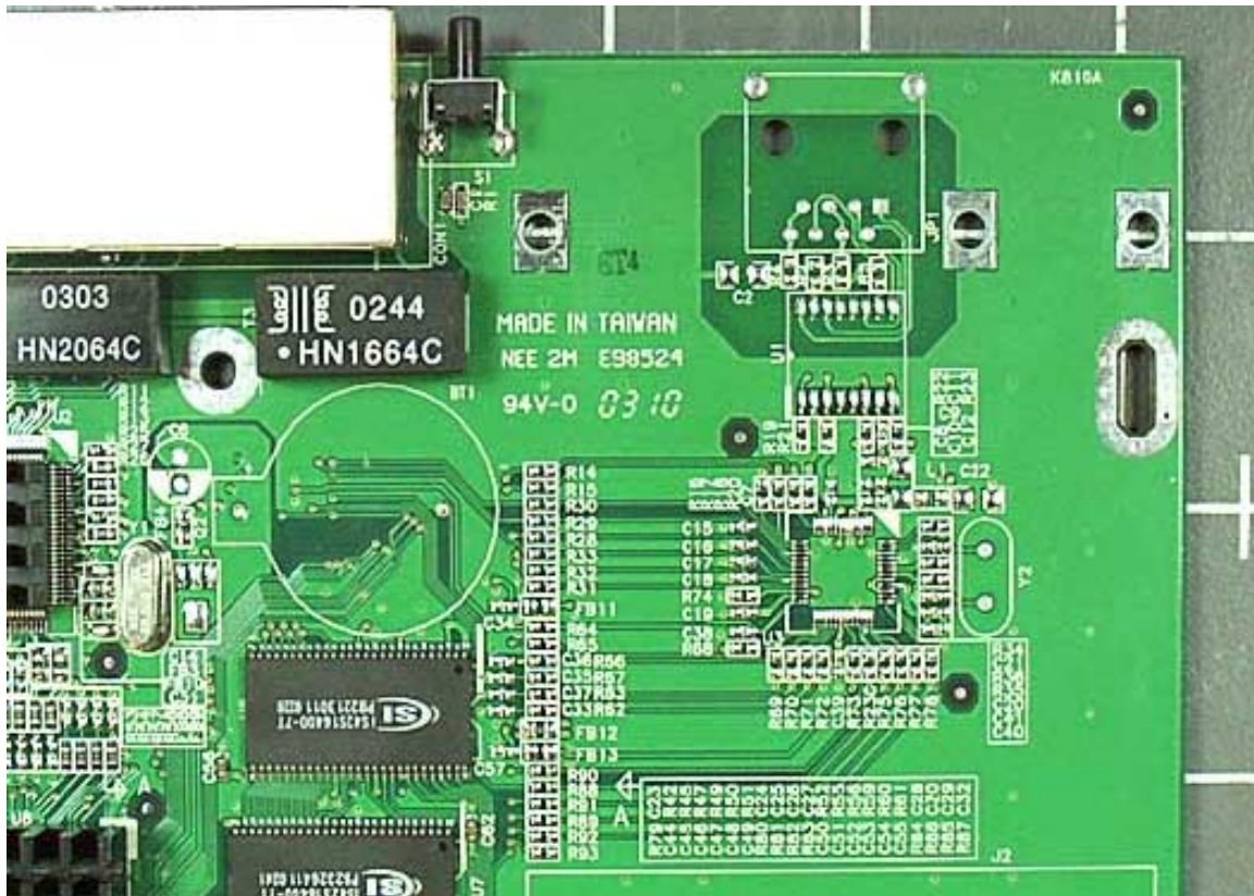
PCB Top #3
