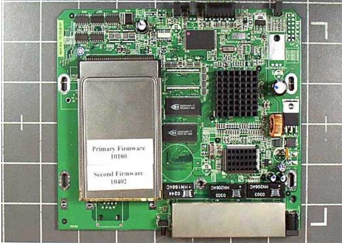
PCB Top with Module
