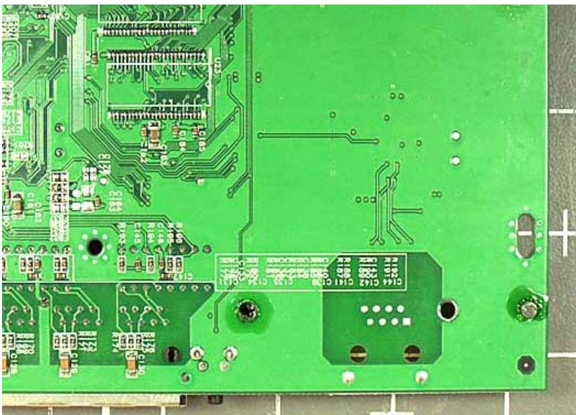
PCB Bottom #1
