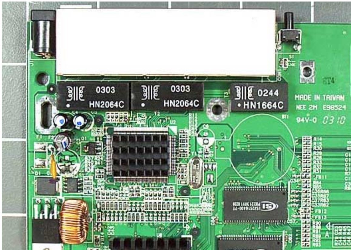
PCB Top #2
