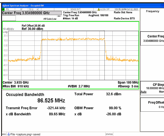
5A_n77(3700-3980MHz) 90M DFT-s-OFDM 16QAM Outer_Full High
