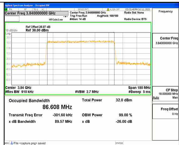
5A_n77(3700-3980MHz) 90M DFT-s-OFDM 64QAM Outer_Full Mid
