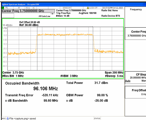
5A_n77(3700-3980MHz) 100M DFT-s-OFDM 16QAM Outer_Full Low
