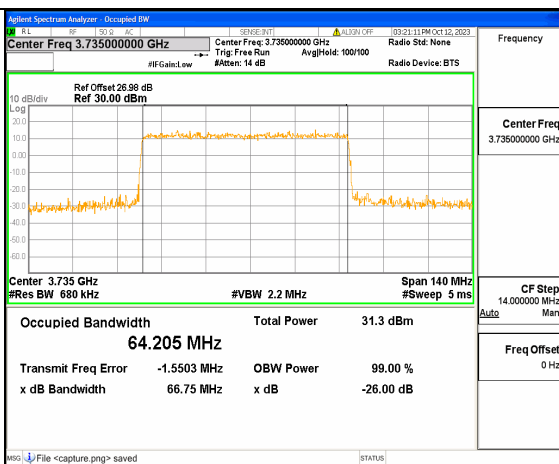
5A_n77(3700-3980MHz) 70M DFT-s-OFDM 16QAM Outer_Full Low
