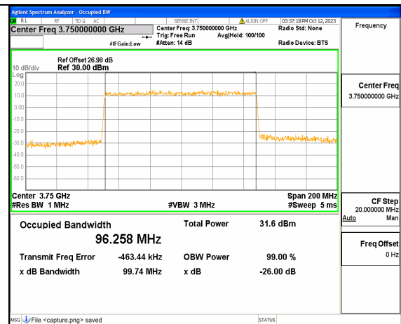
5A_n77(3700-3980MHz) 100M DFT-s-OFDM 64QAM Outer_Full Low
