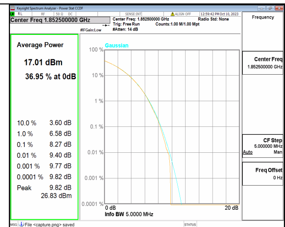
5A_n2 5M CP-OFDM 256QAM Outer_Full Low
