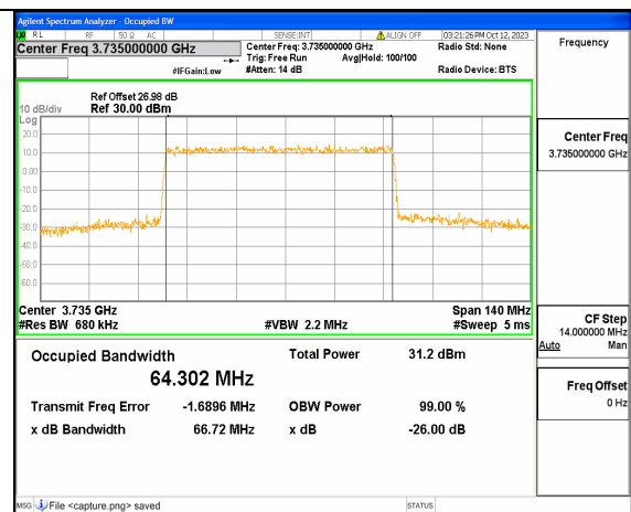
5A_n77(3700-3980MHz) 70M DFT-s-OFDM 64QAM Outer_Full Low
