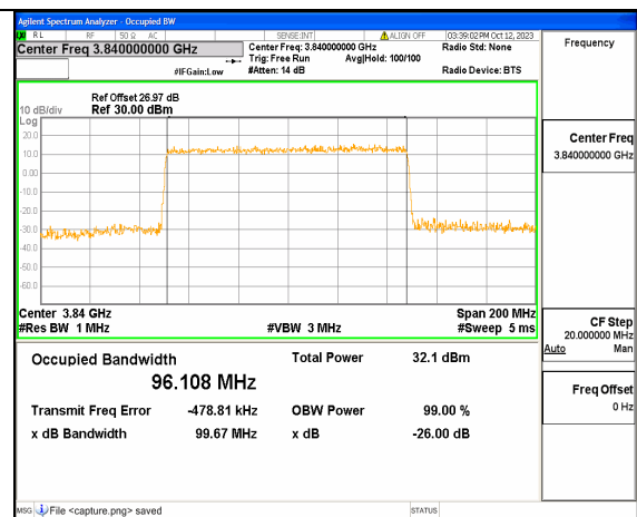
5A_n77(3700-3980MHz) 100M DFT-s-OFDM 64QAM Outer_Full Mid
