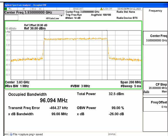
5A_n77(3700-3980MHz) 100M DFT-s-OFDM 64QAM Outer_Full High
