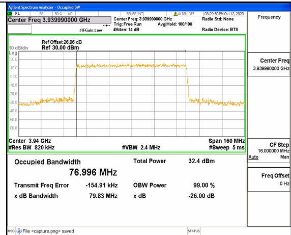
5A_n77(3700-3980MHz) 80M DFT-s-OFDM QPSK Outer_Full High
