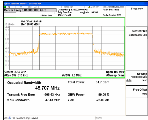
5A_n77(3700-3980MHz) 50M DFT-s-OFDM QPSK Outer_Full Mid
