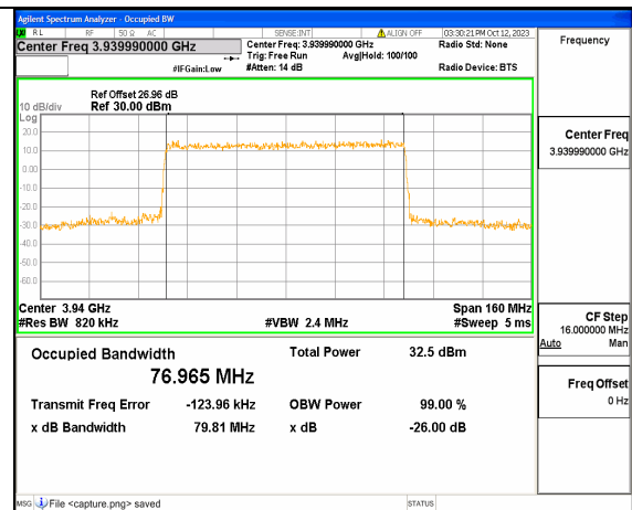
5A_n77(3700-3980MHz) 80M DFT-s-OFDM 64QAM Outer_Full High
