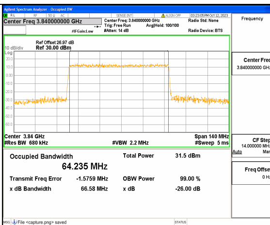
5A_n77(3700-3980MHz) 70M DFT-s-OFDM 16QAM Outer_Full Mid
