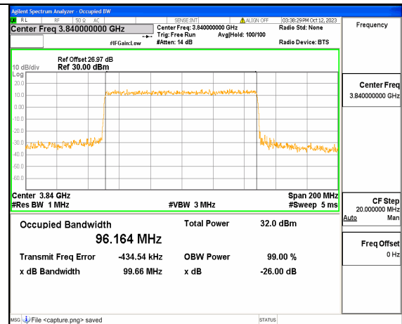
5A_n77(3700-3980MHz) 100M DFT-s-OFDM QPSK Outer_Full Mid
