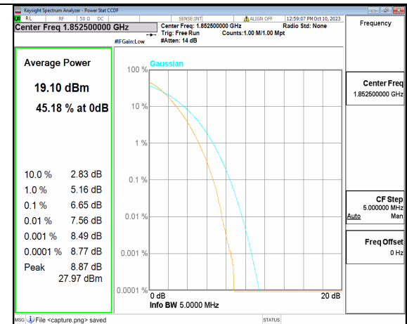
5A_n2 5M DFT-s-OFDM 256QAM Outer_Full Low
