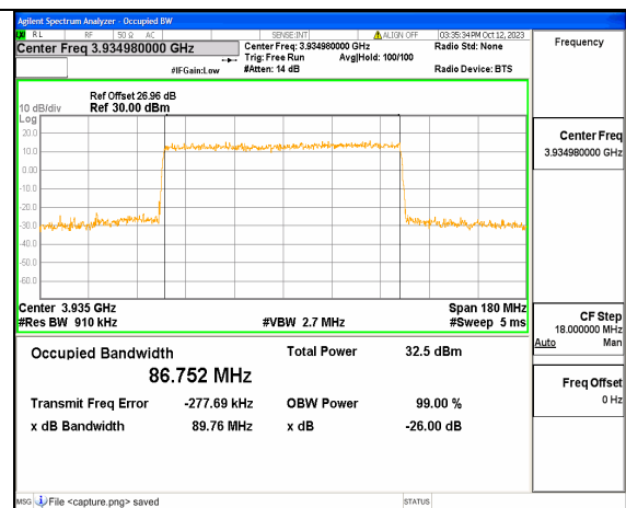
5A_n77(3700-3980MHz) 90M DFT-s-OFDM 64QAM Outer_Full High
