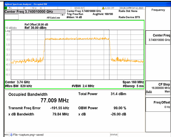
5A_n77(3700-3980MHz) 80M DFT-s-OFDM QPSK Outer_Full Low
