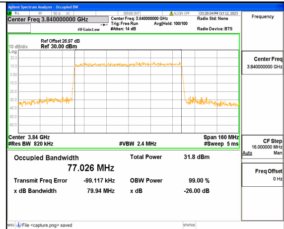
5A_n77(3700-3980MHz) 80M DFT-s-OFDM QPSK Outer_Full Mid
