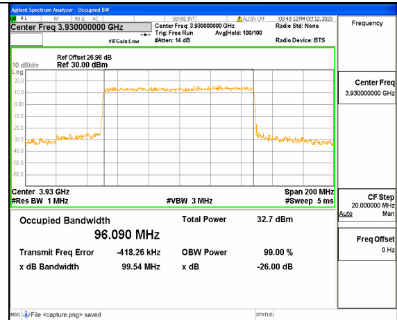
5A_n77(3700-3980MHz) 100M DFT-s-OFDM QPSK Outer_Full High
