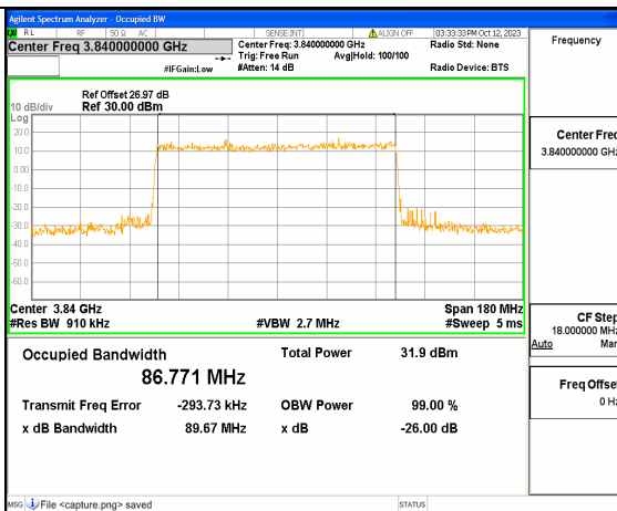
5A_n77(3700-3980MHz) 90M DFT-s-OFDM 16QAM Outer_Full Mid
