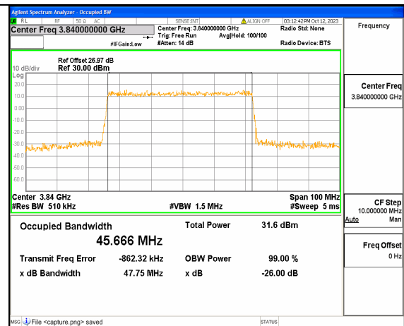
5A_n77(3700-3980MHz) 50M DFT-s-OFDM 64QAM Outer_Full Mid
