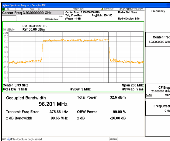
5A_n77(3700-3980MHz) 100M DFT-s-OFDM 16QAM Outer_Full High
