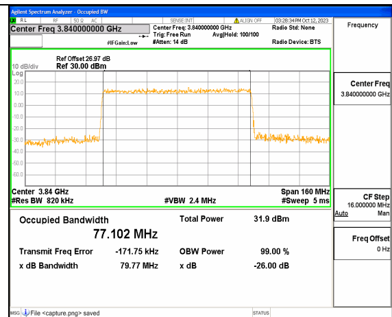
5A_n77(3700-3980MHz) 80M DFT-s-OFDM 64QAM Outer_Full Mid
