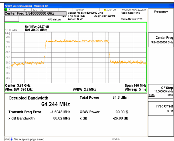
5A_n77(3700-3980MHz) 70M DFT-s-OFDM 64QAM Outer_Full Mid
