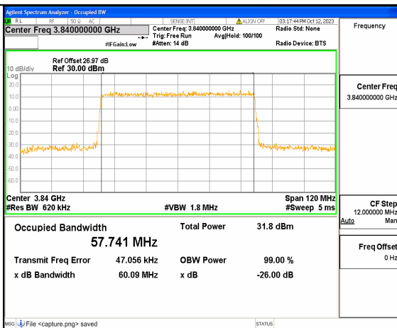
5A_n77(3700-3980MHz) 60M DFT-s-OFDM 16QAM Outer_Full Mid
