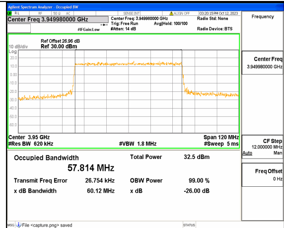
5A_n77(3700-3980MHz) 60M CP-OFDM QPSK Outer_Full High
