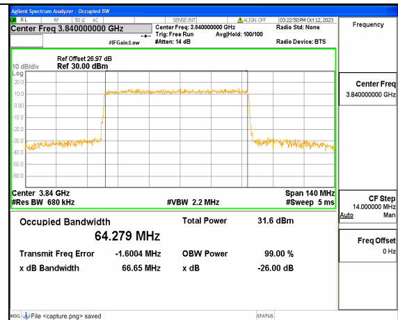
5A_n77(3700-3980MHz) 70M DFT-s-OFDM QPSK Outer_Full Mid
