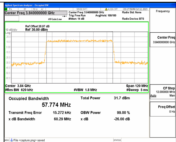
5A_n77(3700-3980MHz) 60M DFT-s-OFDM 64QAM Outer_Full Mid
