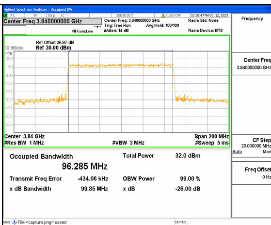
5A_n77(3700-3980MHz) 100M DFT-s-OFDM 16QAM Outer_Full Mid
