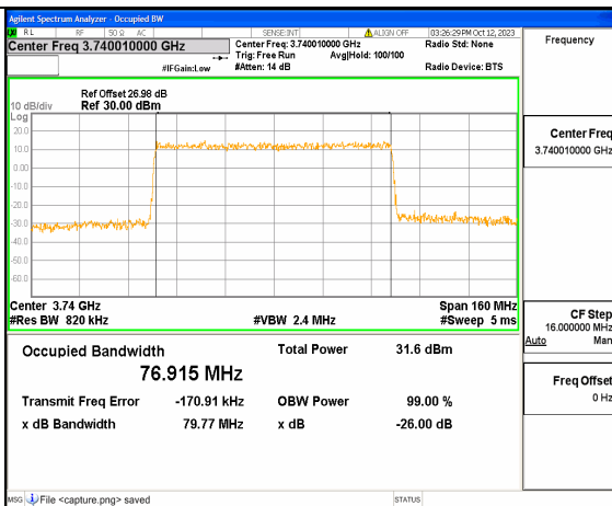
5A_n77(3700-3980MHz) 80M DFT-s-OFDM 16QAM Outer_Full Low
