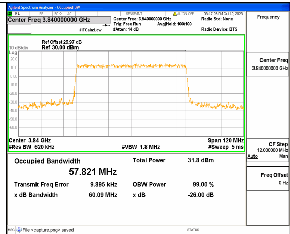
5A_n77(3700-3980MHz) 60M DFT-s-OFDM QPSK Outer_Full Mid
