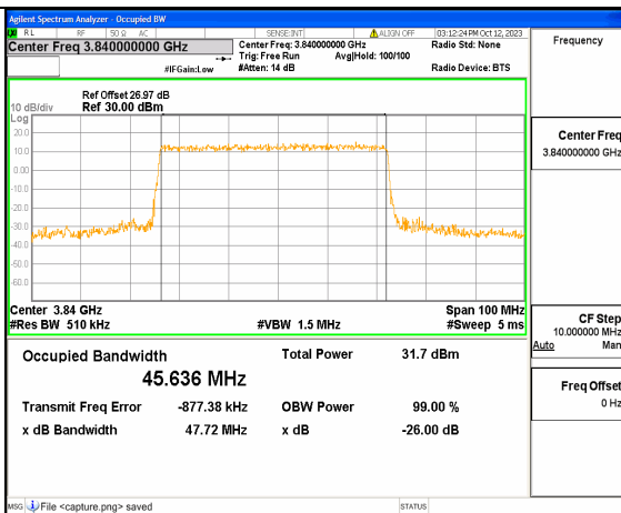
5A_n77(3700-3980MHz) 50M DFT-s-OFDM 16QAM Outer_Full Mid
