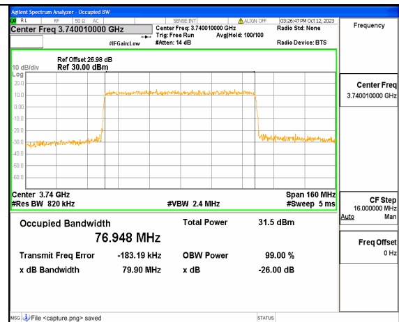
5A_n77(3700-3980MHz) 80M DFT-s-OFDM 64QAM Outer_Full Low
