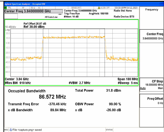
5A_n77(3700-3980MHz) 90M DFT-s-OFDM QPSK Outer_Full Mid
