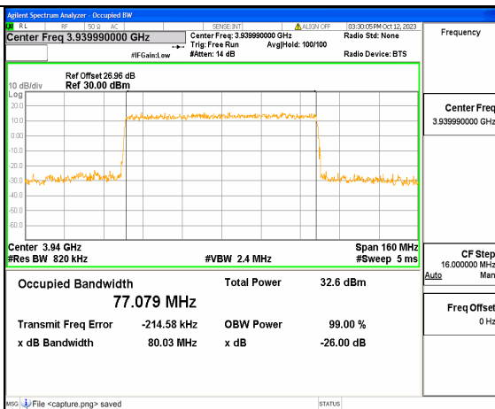
5A_n77(3700-3980MHz) 80M DFT-s-OFDM 16QAM Outer_Full High
