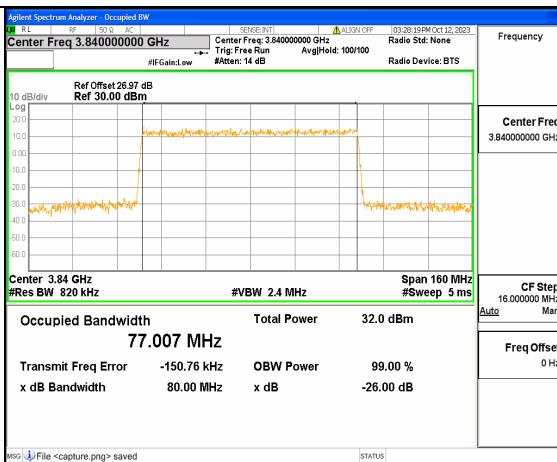
5A_n77(3700-3980MHz) 80M DFT-s-OFDM 16QAM Outer_Full Mid
