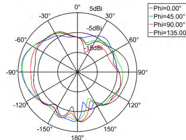
radiation pattern of the antenna realized gain (E_Total, Freq = 2500.00 MHz)
