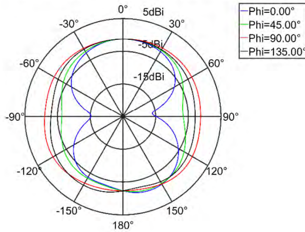
radiation pattern of the antenna realized gain (E_Total, Freq = 738.00 MHz)
