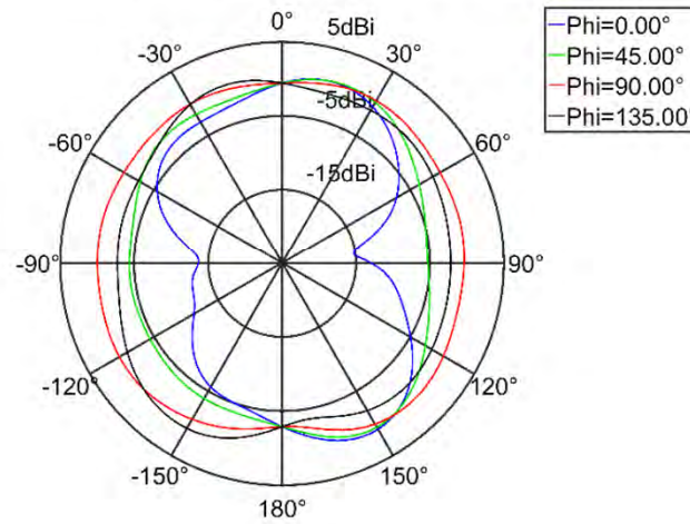
radiation pattern of the antenna realized gain (E_Total, Freq = 849.00 MHz)
