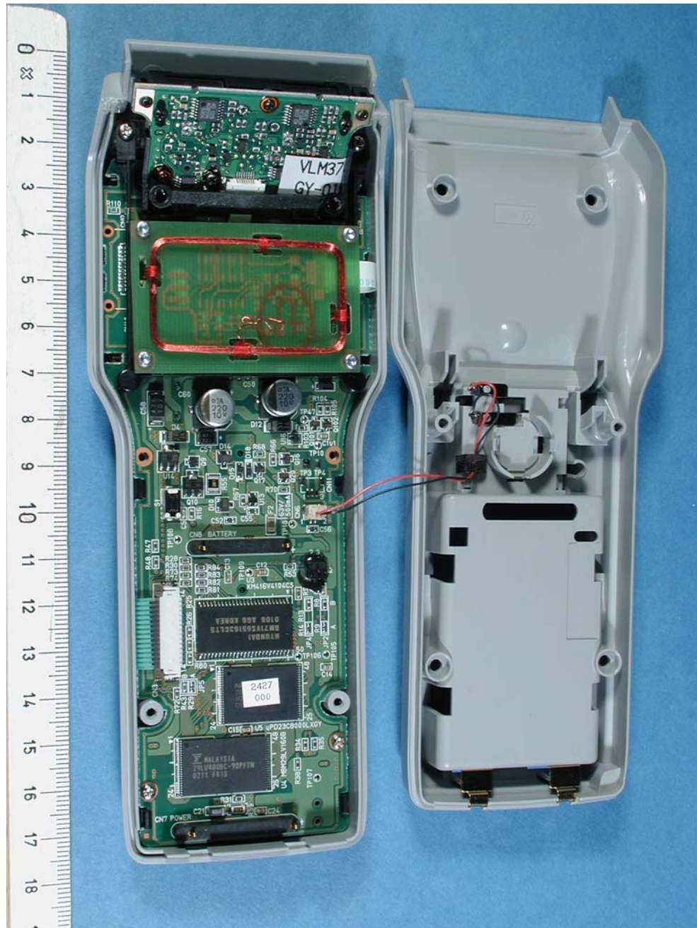
Internal view of equipment
