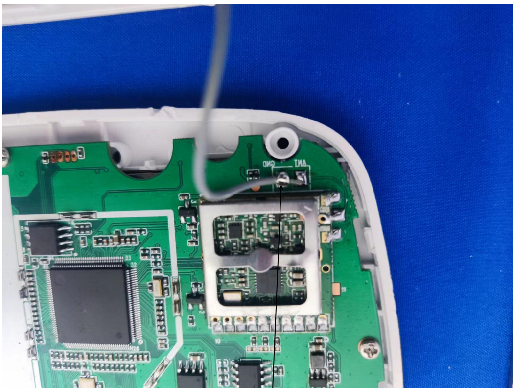
Integral Antenna
